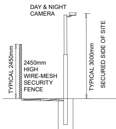
CCTV CAMERA DETAILS - TYICAL SECTION
