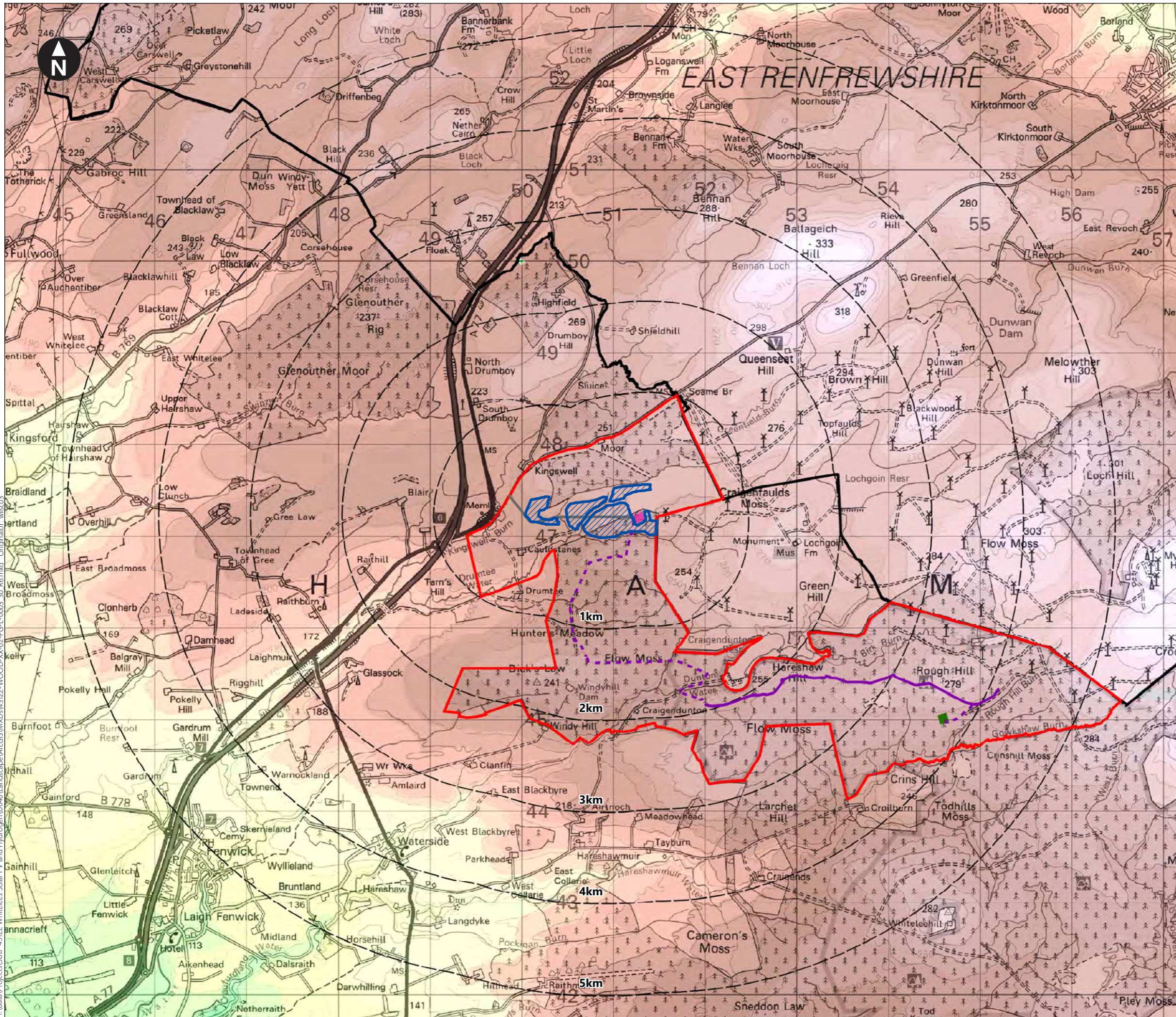
Figure 7.3 Topography
