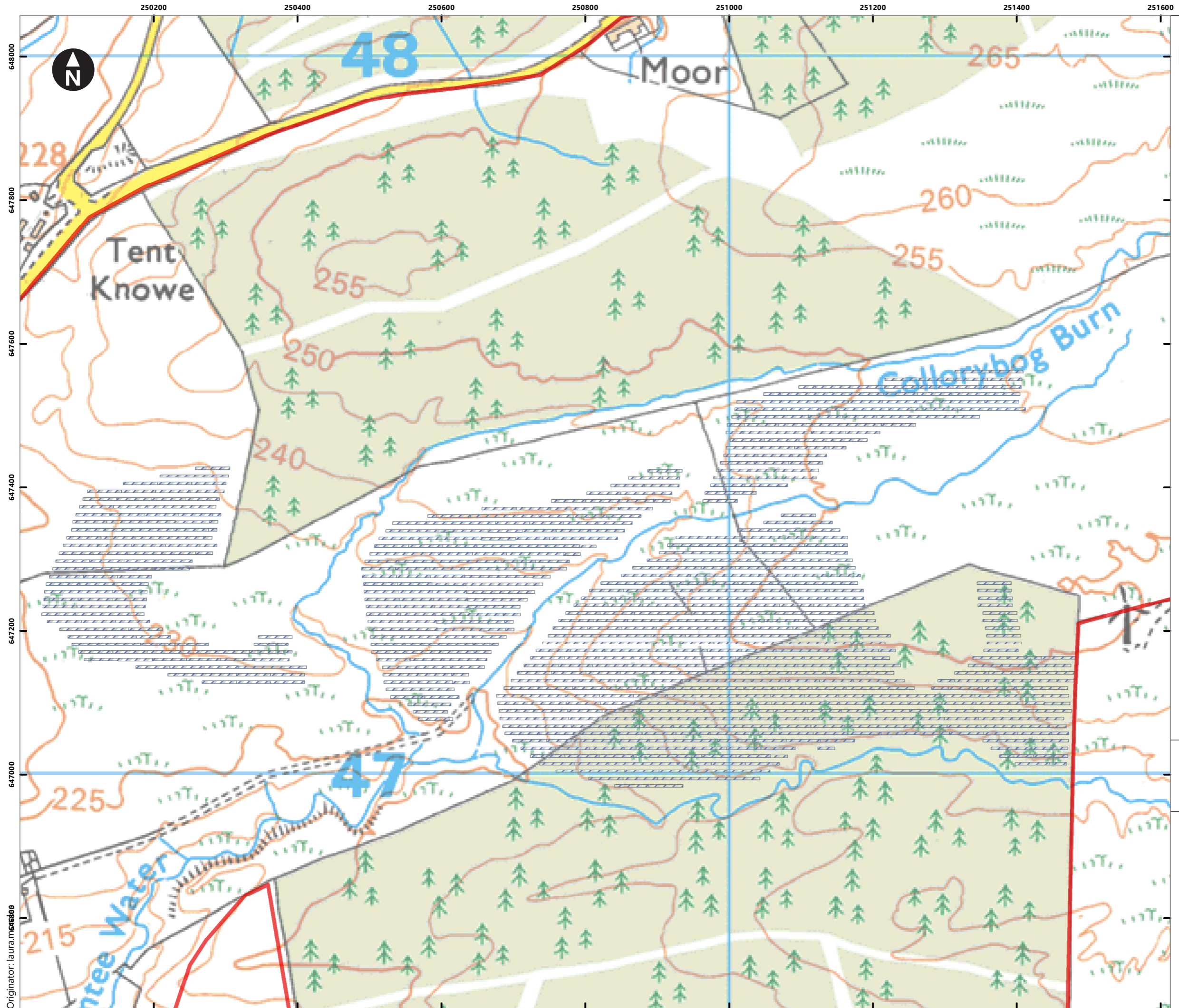
Figure 1.6 Solar PV Farm Proposed Layout
