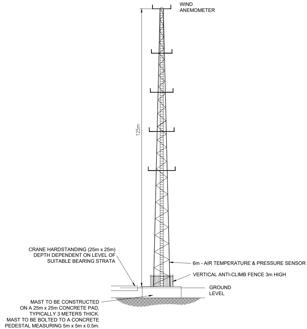
TYPICAL MET MAST DETAIL
