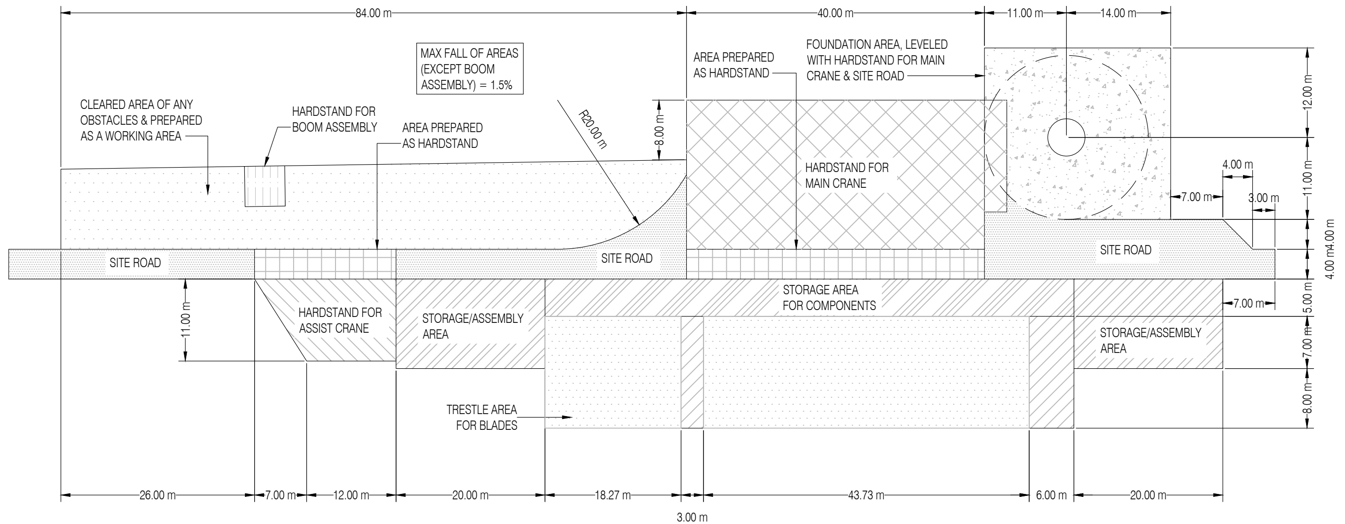
CRANE HARDSTANDING DETAILS SCALE 1:500
