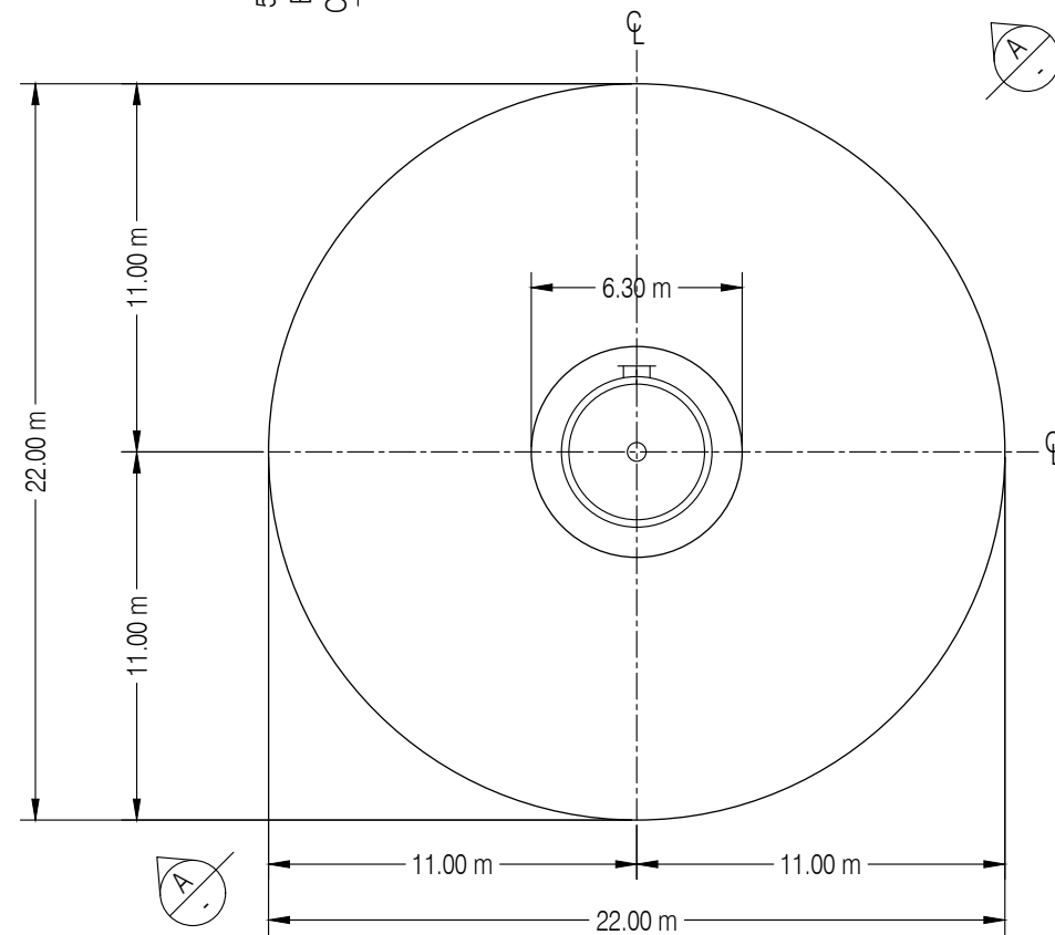
GENERAL PLAN SCALE 1:250
