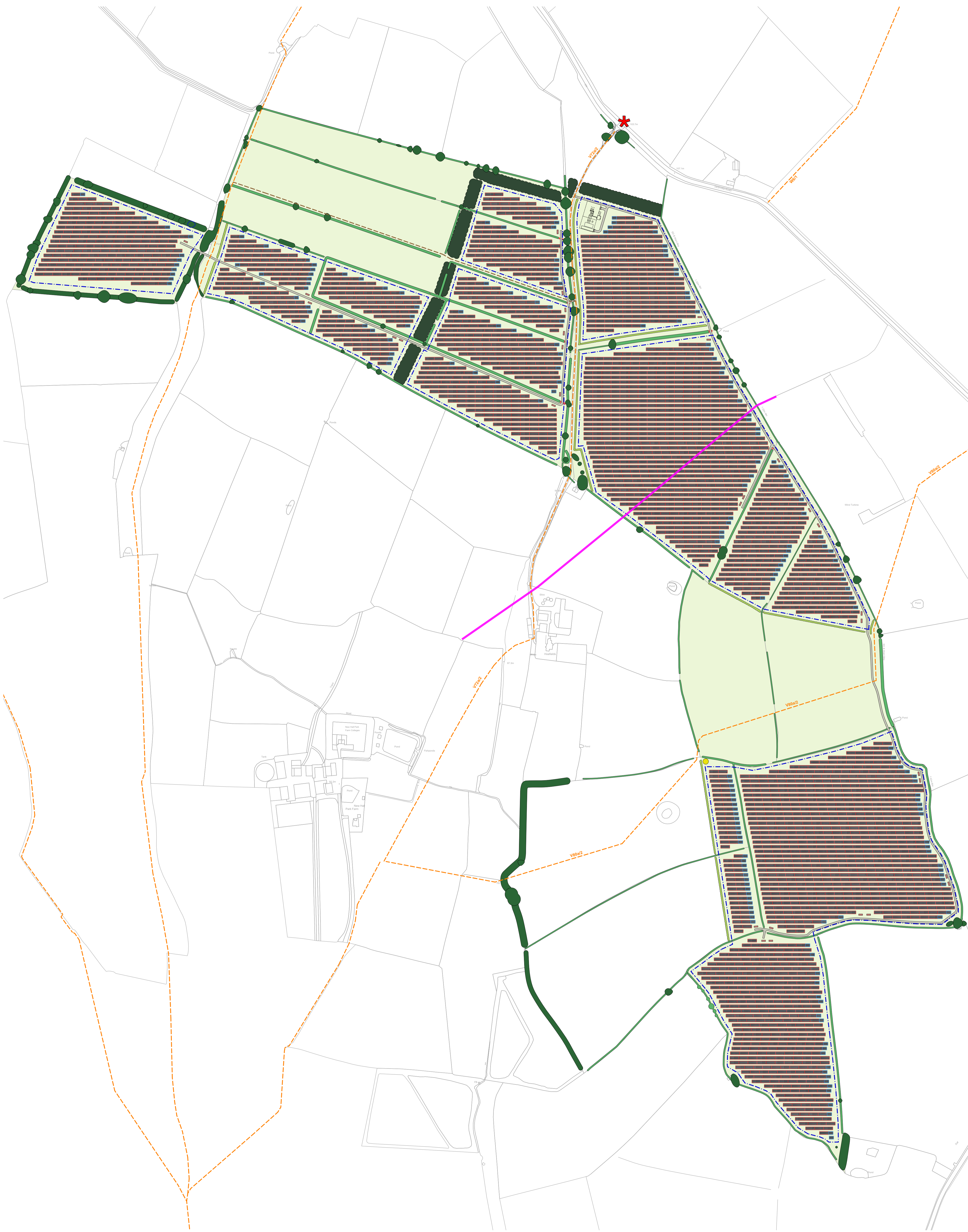
FIGURE 6.2 Site Layout and Planting Proposals
