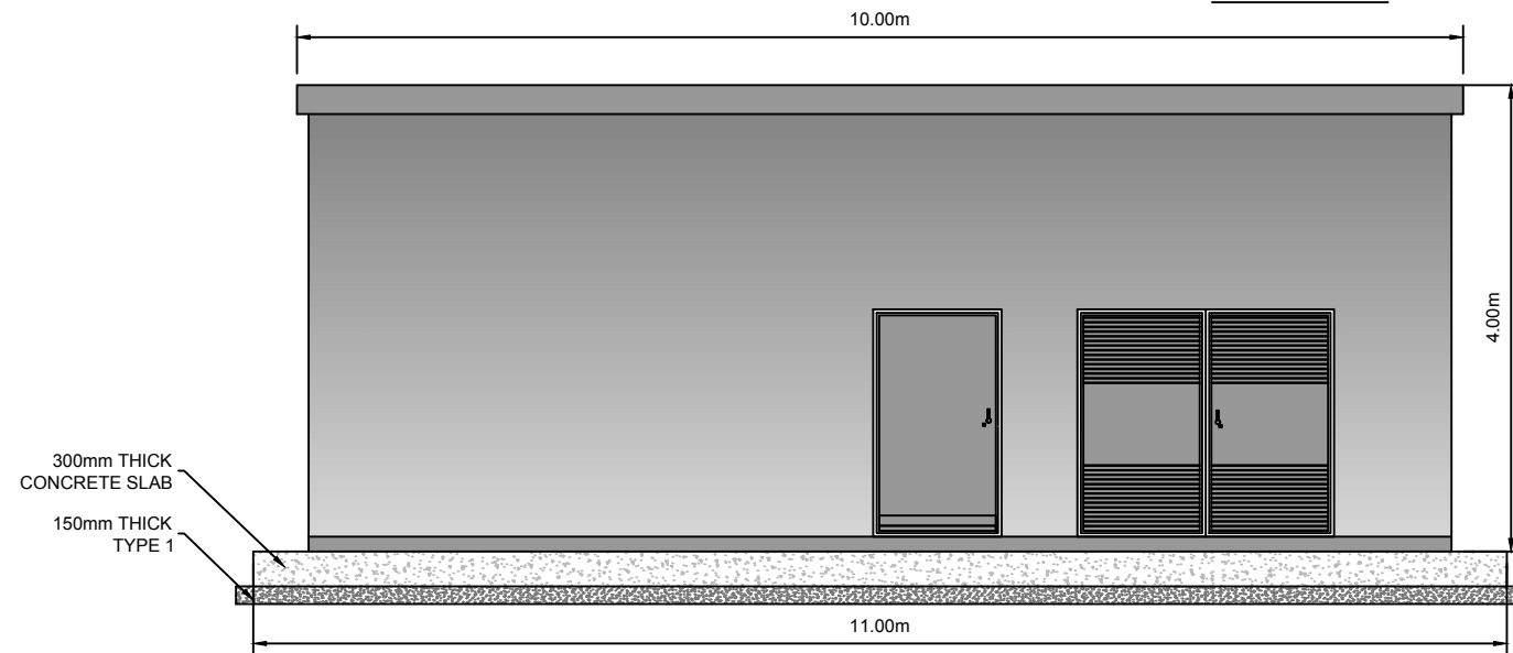
SIDE VIEW
