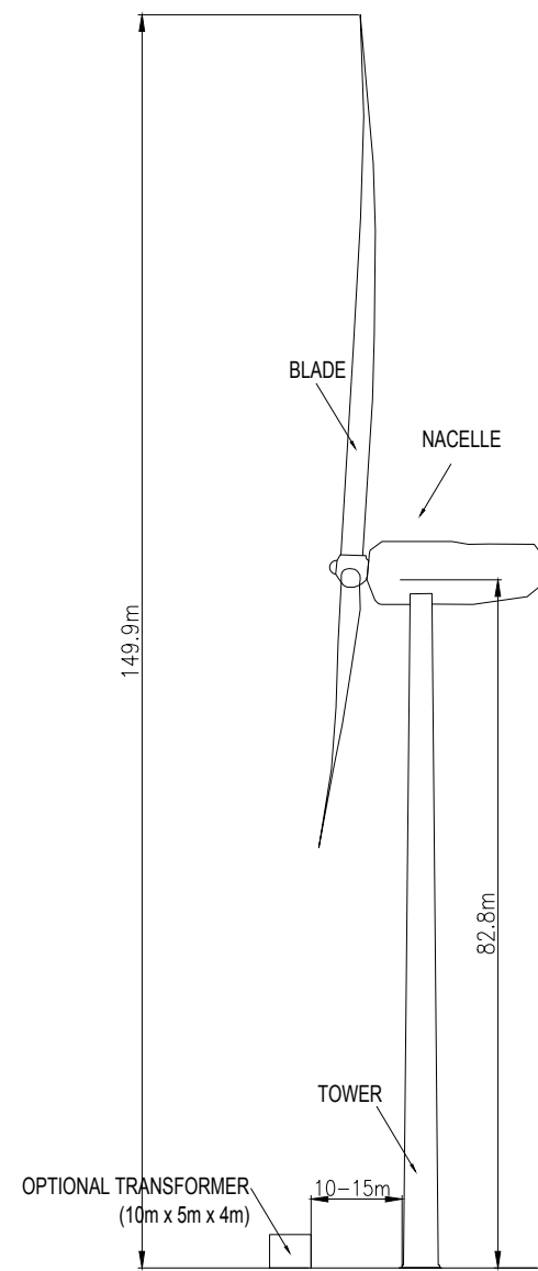
SIDE ELEVATION (1:500)
