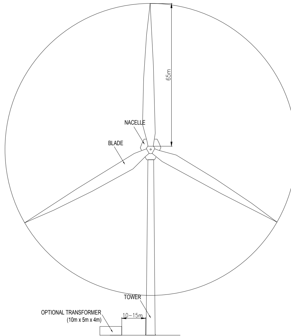
FRONT ELEVATION (1:500)
