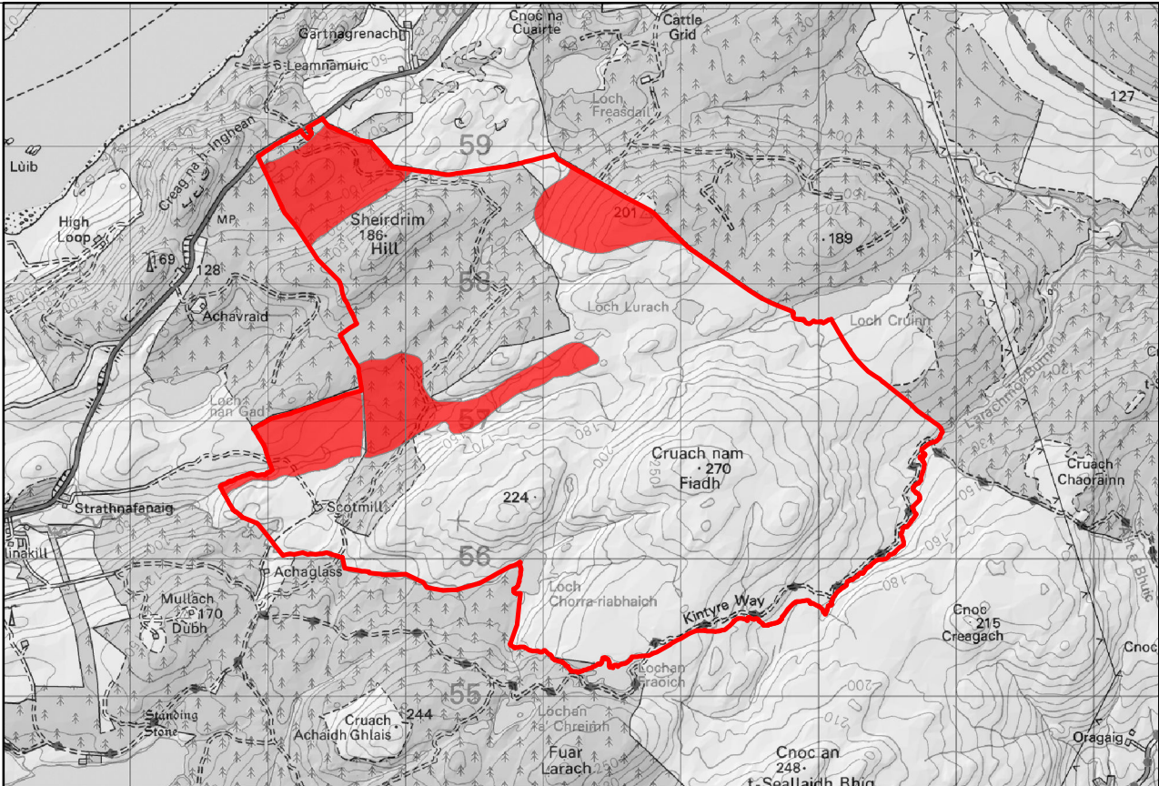
Superficial Aquifers
