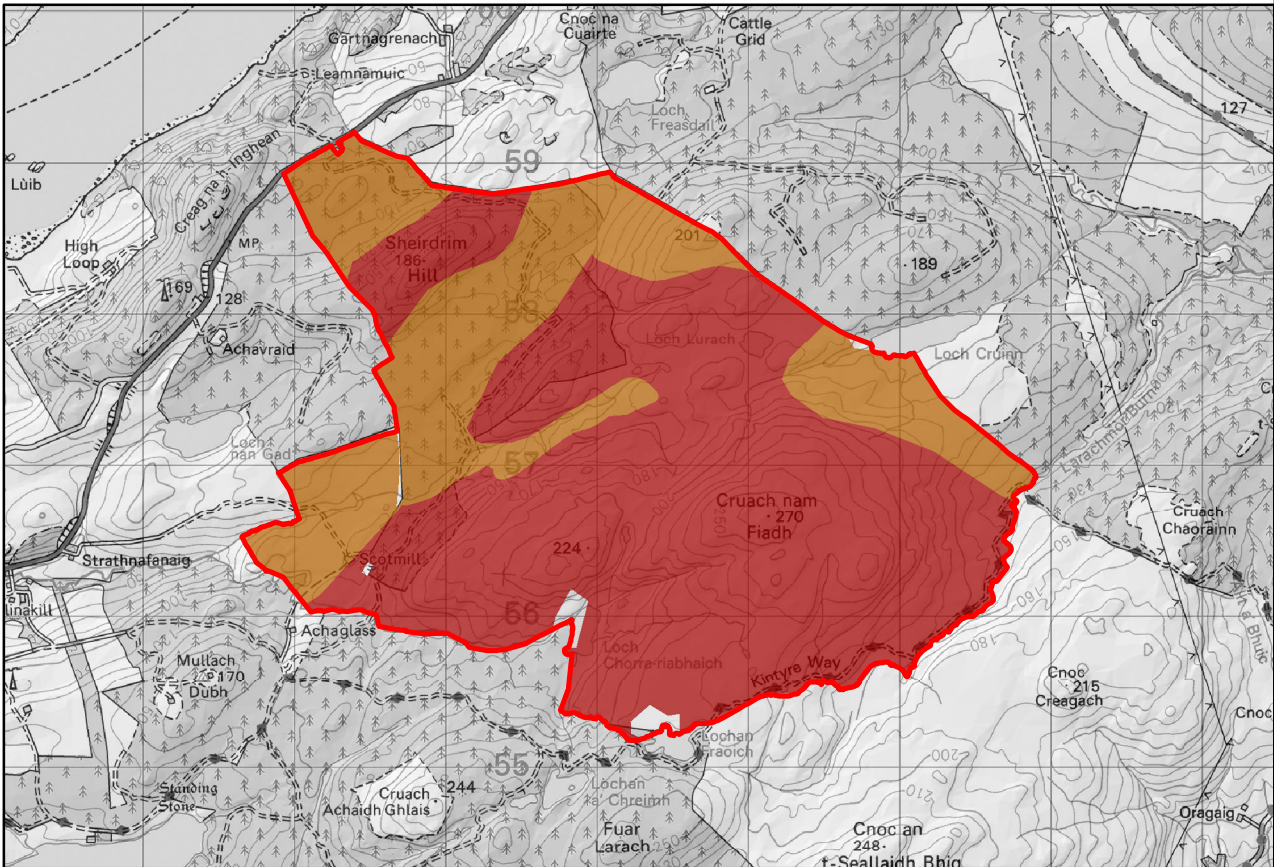
Groundwater Vulnerability in the Uppermost Aquifer
