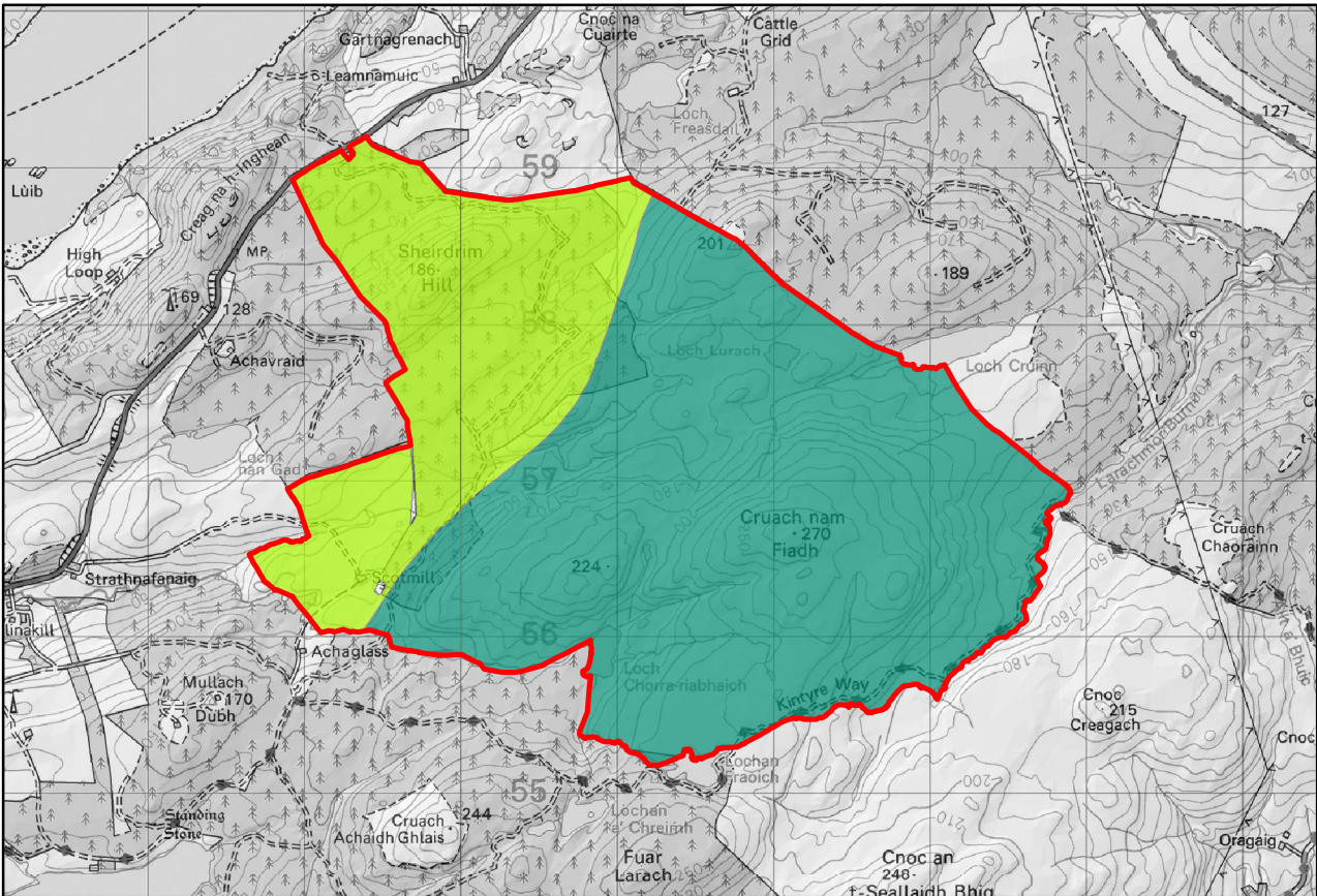
Bedrock Aquifers
