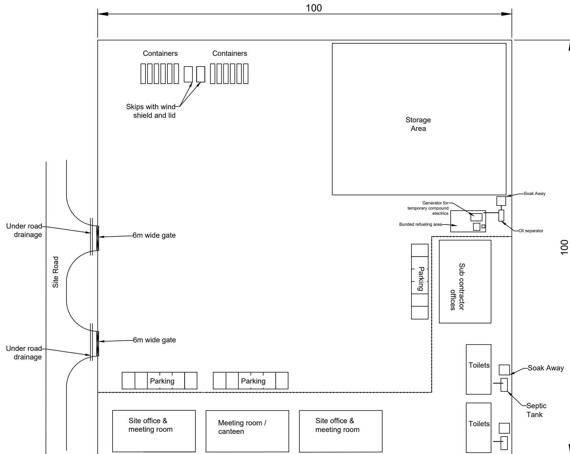
Typical Main Construction Compound Layout
