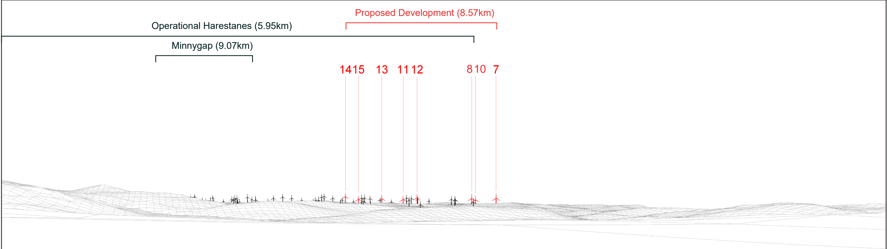
Layout F (8 turbines and 200m tip height)
