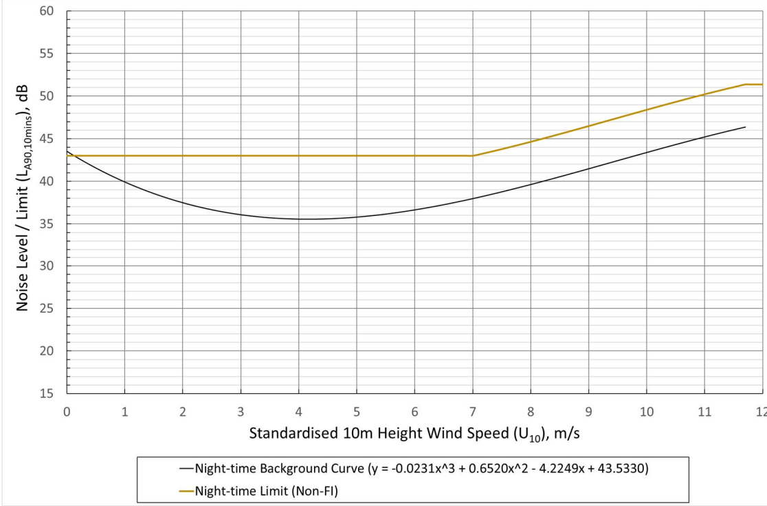
Graph 9.8.6: Location C Lamphitt – Night-time Cumulative Noise Limit, dB(A) versus Wind Speed (m/s)
