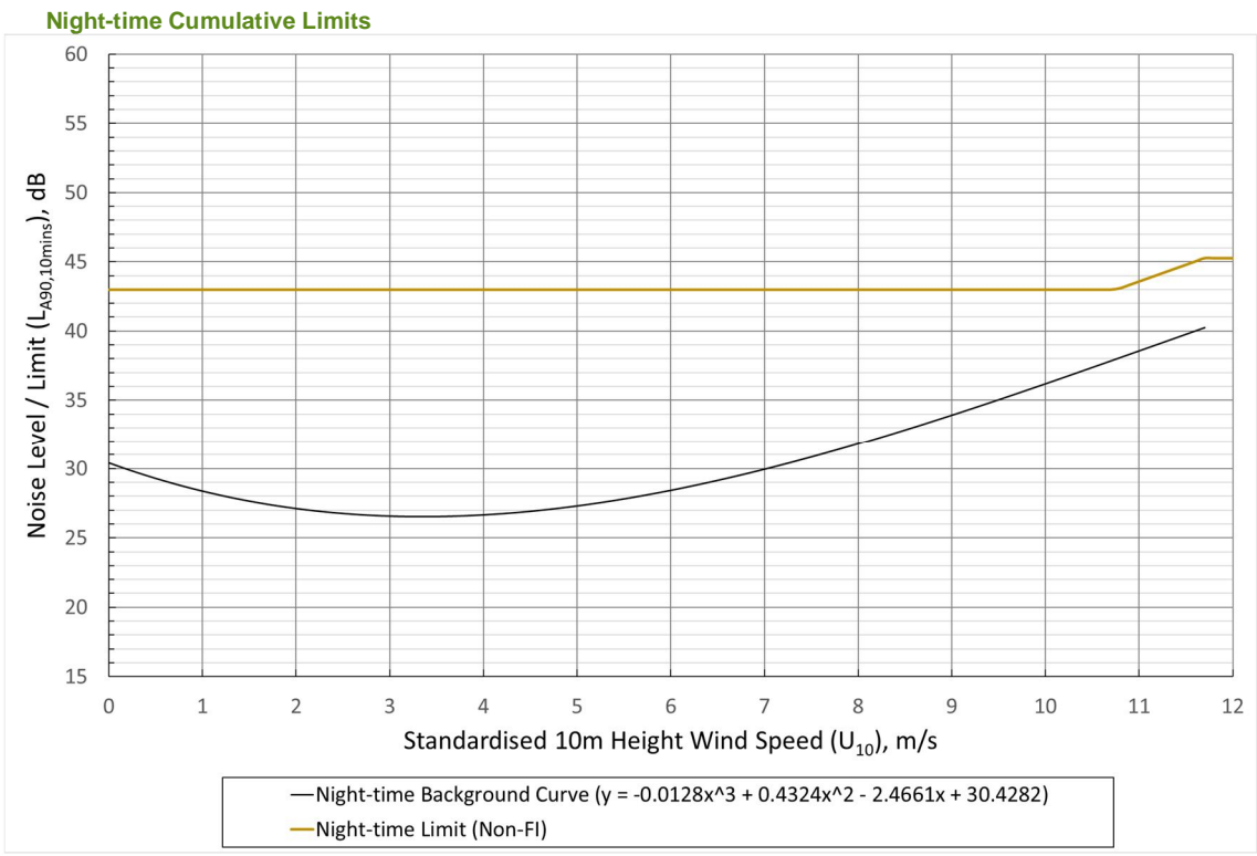
Graph 9.8.4: Location B Burrancehill Cottage – Night-time Cumulative Noise Limit, dB(A) versus Wind Speed (m/s)
