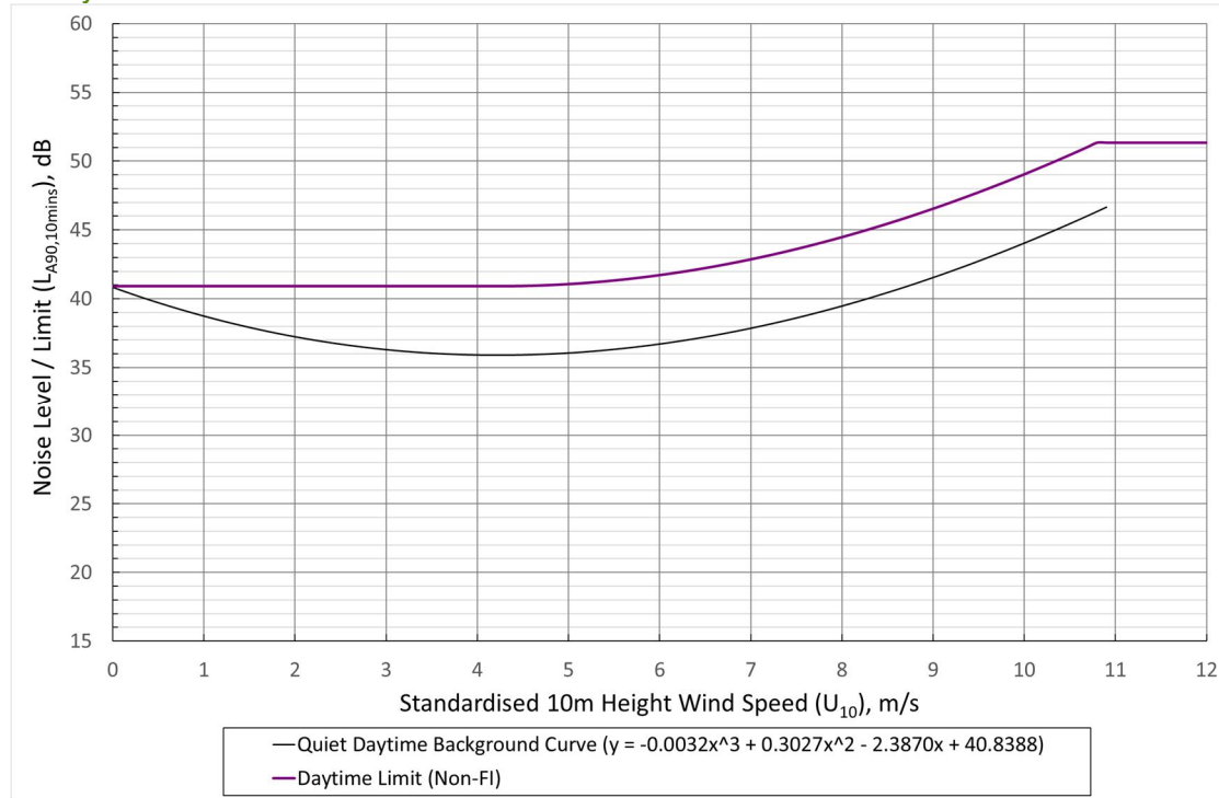
Graph 9.8.5: Location C Lamphitt – Daytime Cumulative Noise Limit, dB(A) versus Wind Speed (m/s)
