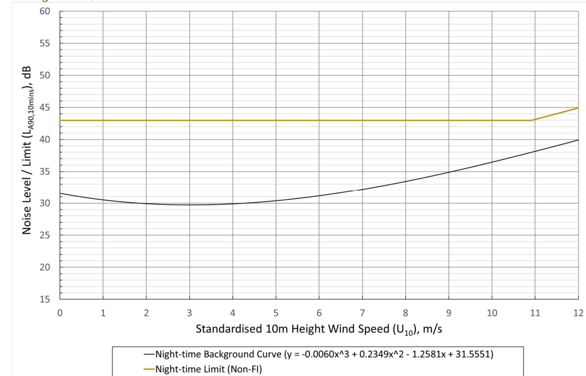
Graph 9.8.8: Location D Glenview – Night-time Cumulative Noise Limit, dB(A) versus Wind Speed (m/s)
