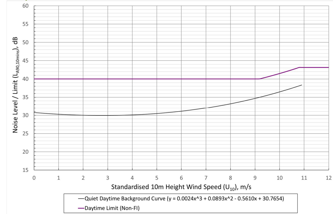
Graph 9.8.7: Location D Glenview – Daytime Cumulative Noise Limit, dB(A) versus Wind Speed (m/s)
