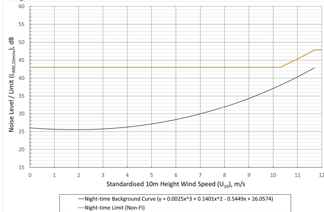
Graph 9.8.2: Location A Mollin Farm – Night-time Cumulative Noise Limit, dB(A) versus Wind Speed (m/s)
