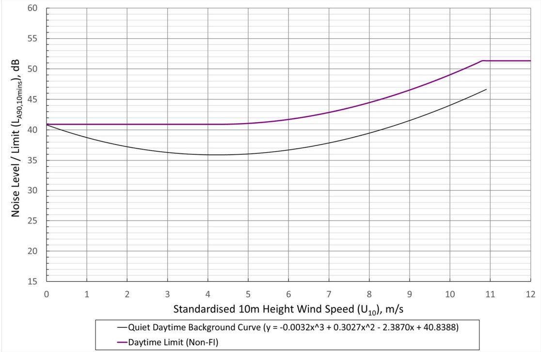
Graph 9.8.5: Location C Lamphitt – Daytime Cumulative Noise Limit, dB(A) versus Wind Speed (m/s)
