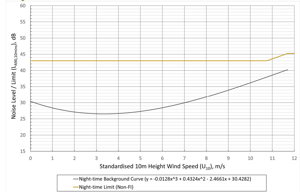
Graph 9.8.4: Location B Burrancehill Cottage – Night-time Cumulative Noise Limit, dB(A) versus Wind Speed (m/s)
