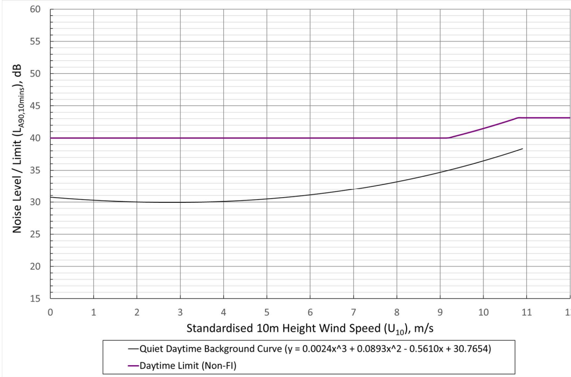
Graph 9.8.7: Location D Glenview – Daytime Cumulative Noise Limit, dB(A) versus Wind Speed (m/s)
