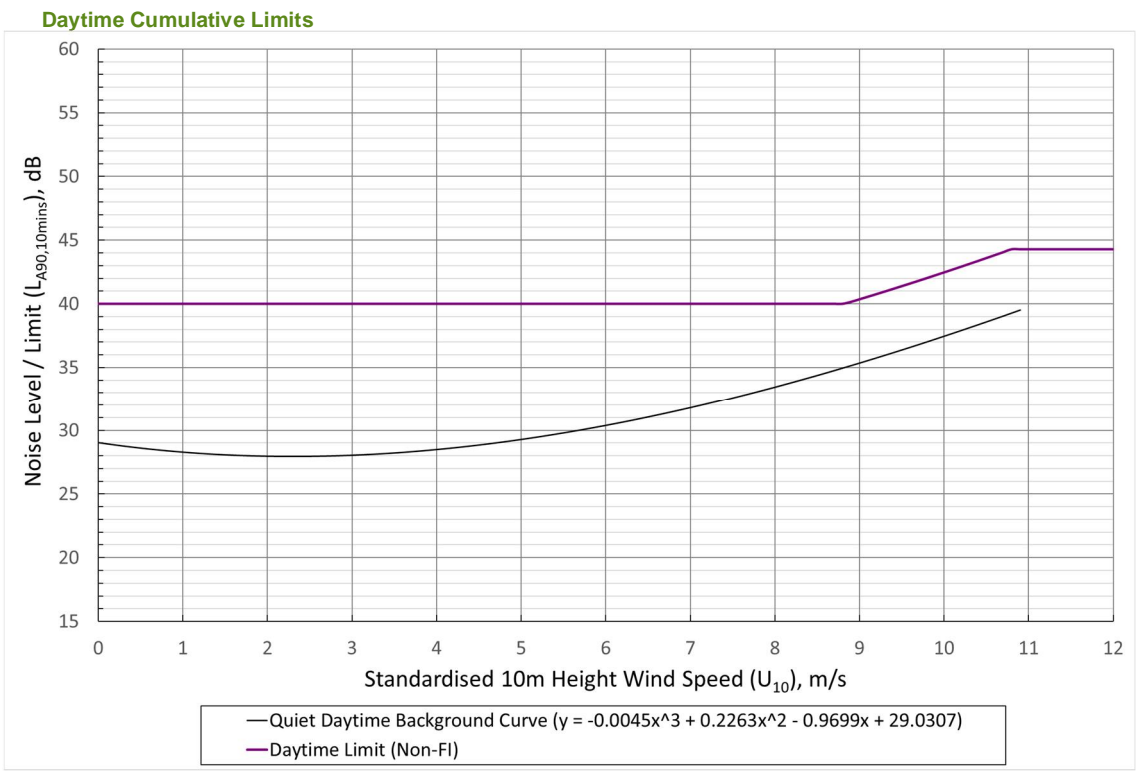
Graph 9.8.3: Location B Burrancehill Cottage – Daytime Cumulative Noise Limit, dB(A) versus Wind Speed (m/s)
