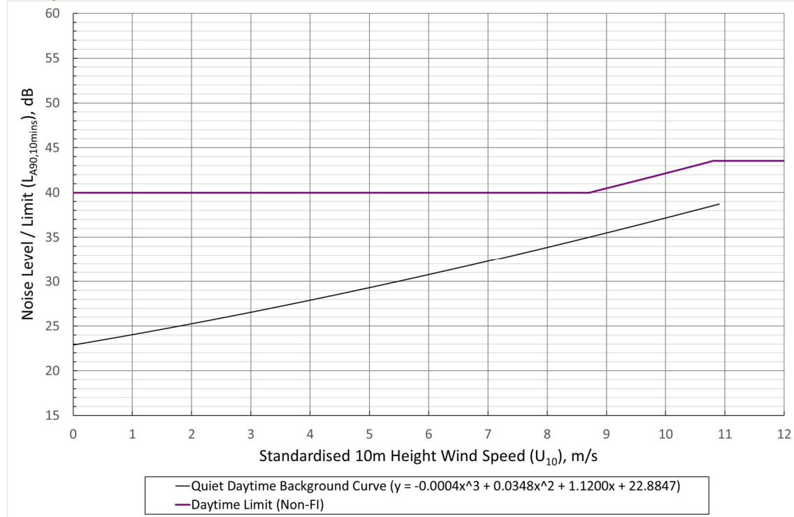
Graph 9.8.1: Location A Mollin Farm – Daytime Cumulative Noise Limit, dB(A) versus Wind Speed (m/s)
