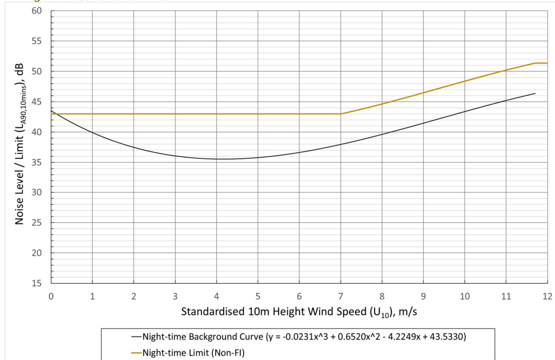
Graph 9.8.6: Location C Lamphitt – Night-time Cumulative Noise Limit, dB(A) versus Wind Speed (m/s)
