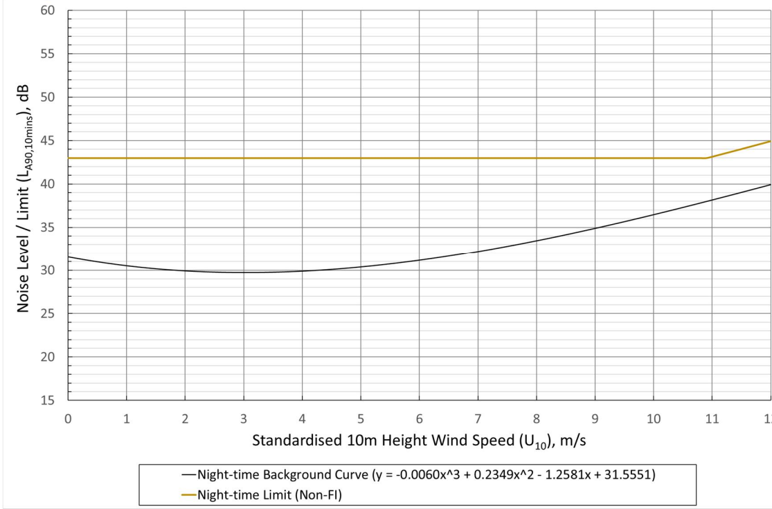
Graph 9.8.8: Location D Glenview – Night-time Cumulative Noise Limit, dB(A) versus Wind Speed (m/s)
