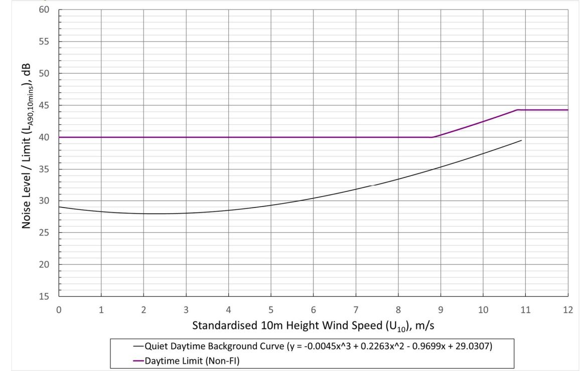
Graph 9.8.3: Location B Burrancehill Cottage – Daytime Cumulative Noise Limit, dB(A) versus Wind Speed (m/s)
