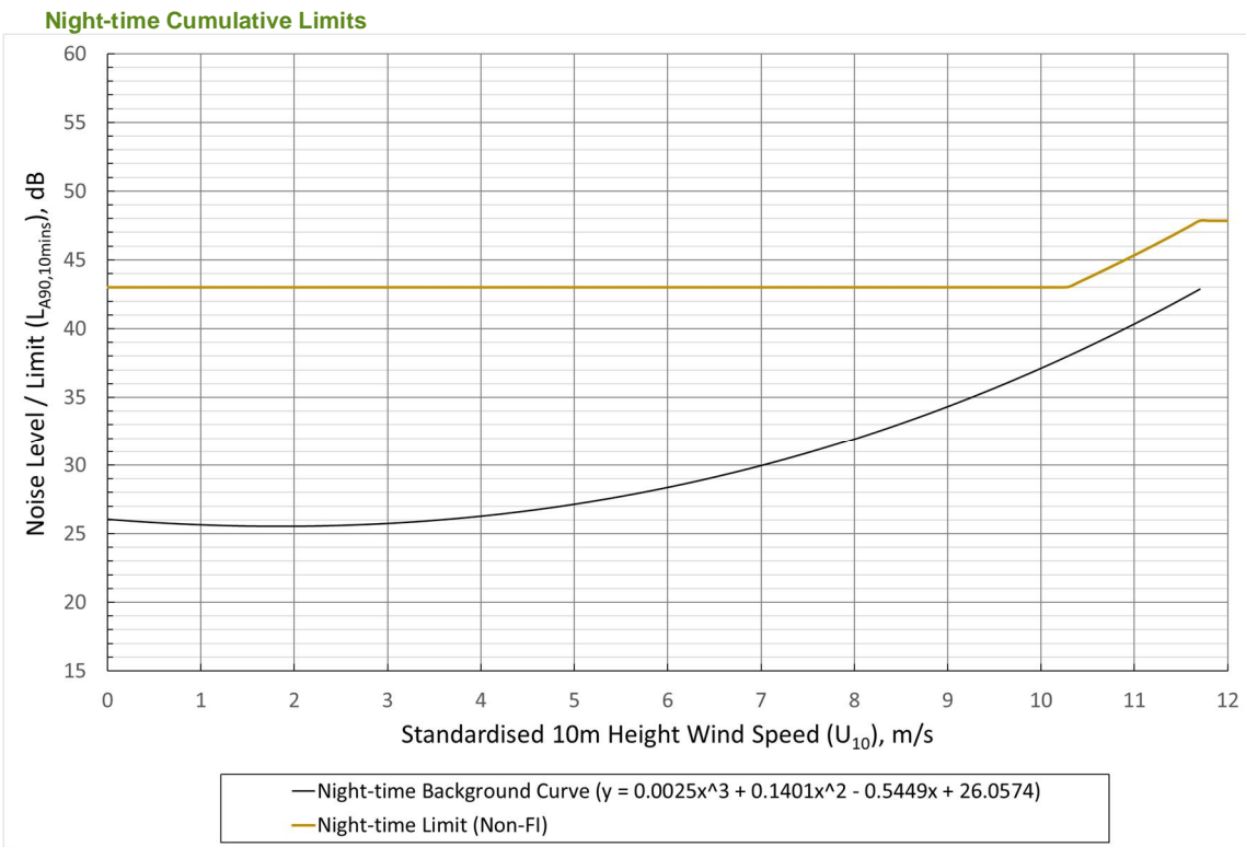
Graph 9.8.2: Location A Mollin Farm – Night-time Cumulative Noise Limit, dB(A) versus Wind Speed (m/s)
