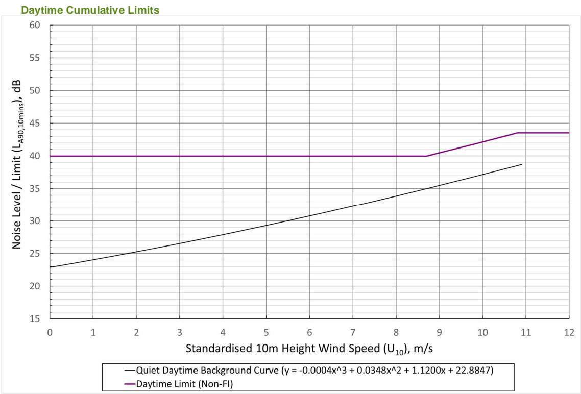
Graph 9.8.1: Location A Mollin Farm – Daytime Cumulative Noise Limit, dB(A) versus Wind Speed (m/s)
