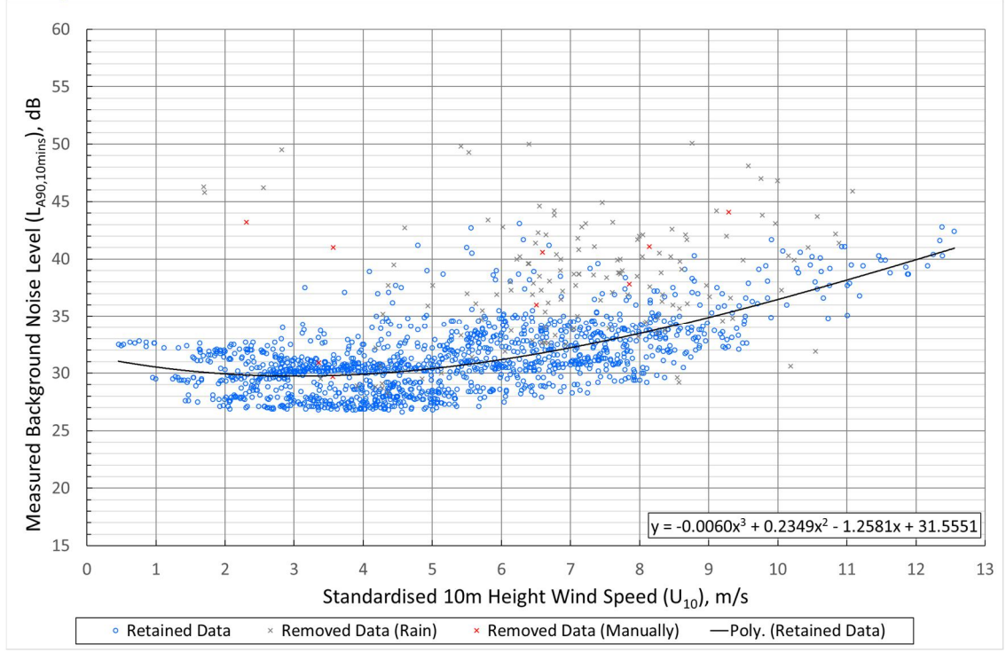
Graph 9.5.8: Location D Glenview – Night-time Daytime Background Noise (dB(A)) versus Wind Speed (m/s)
