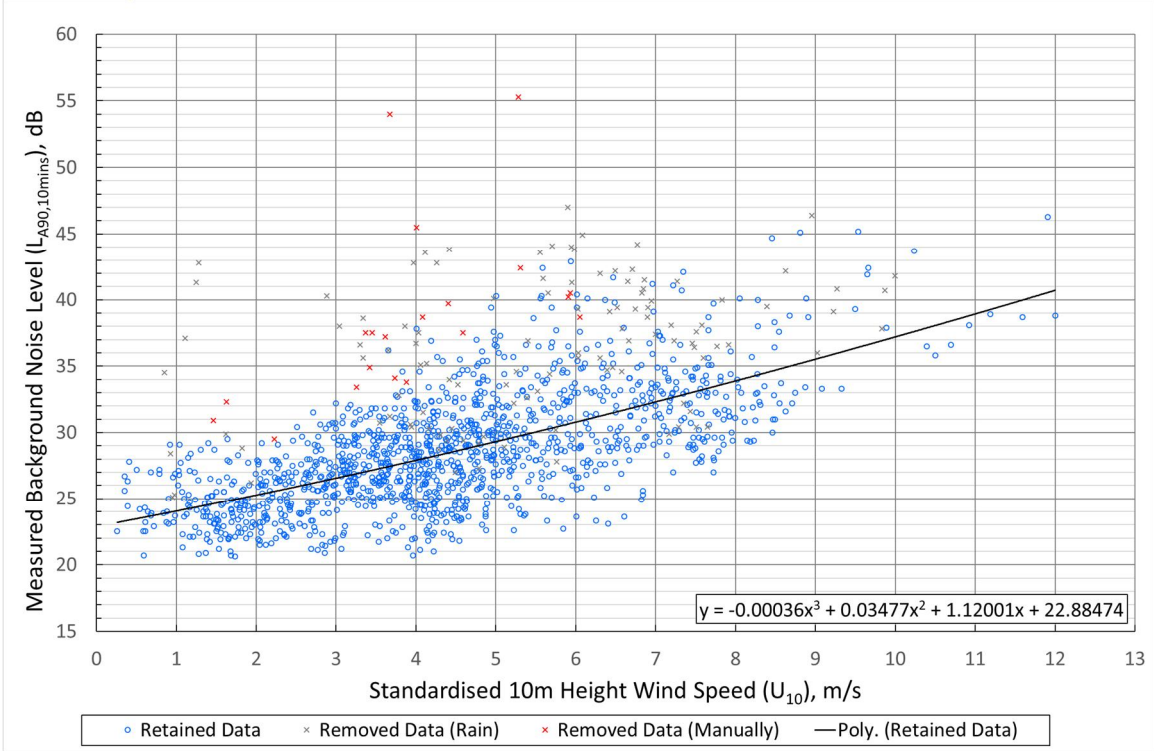
Graph 9.5.1: Location A Mollin Farm – Quiet Daytime Background Noise (dB(A)) versus Wind Speed (m/s)
