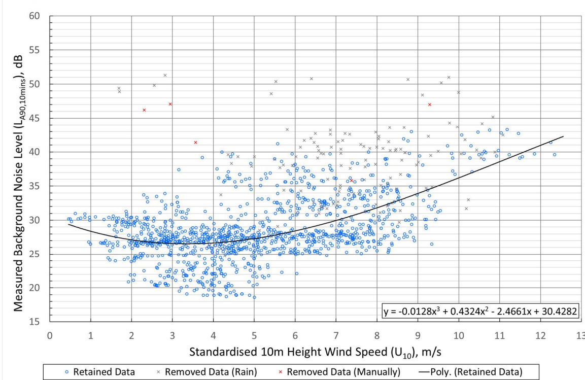
Graph 9.5.4: Location B Burrancehill Cottage – Night-time Daytime Background Noise (dB(A)) versus Wind Speed (m/s)
