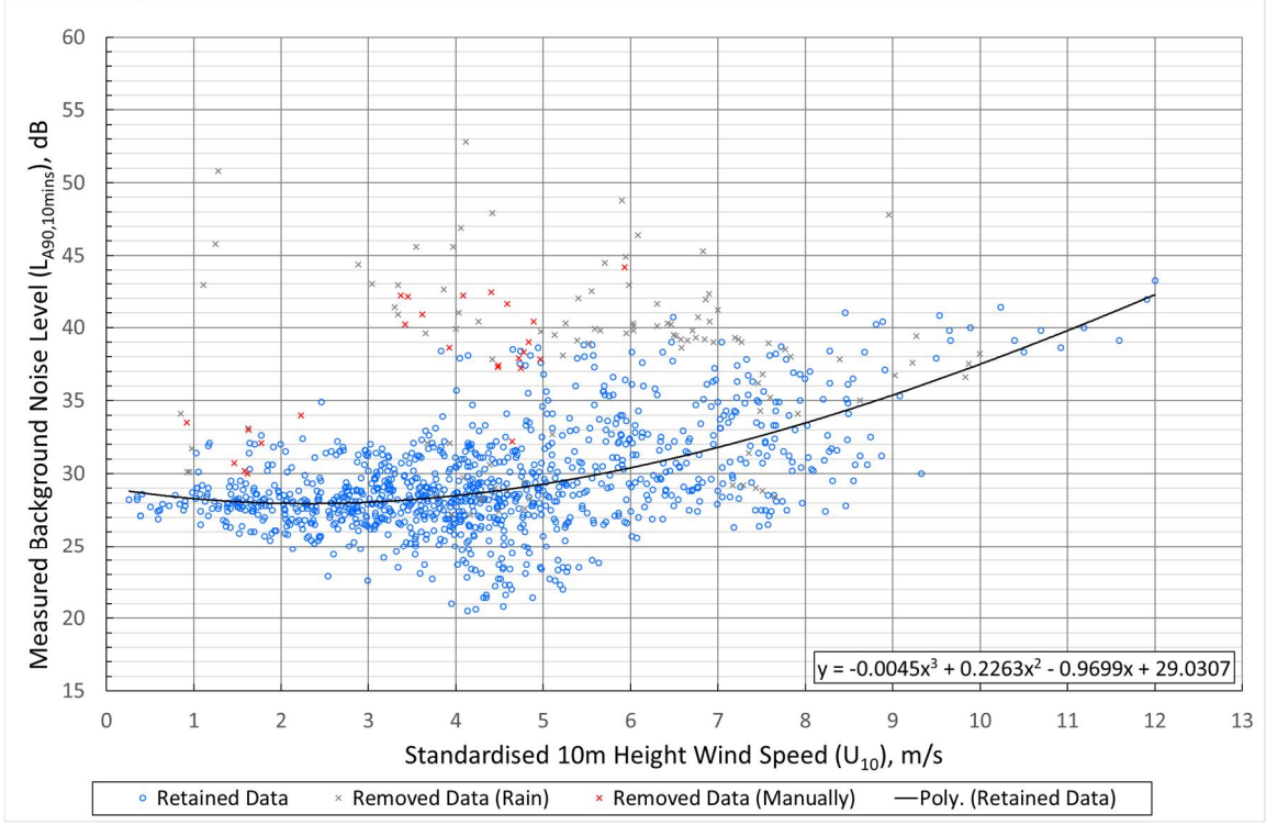
Graph 9.5.3: Location B Burrancehill Cottage – Quiet Daytime Background Noise (dB(A)) versus Wind Speed (m/s)
