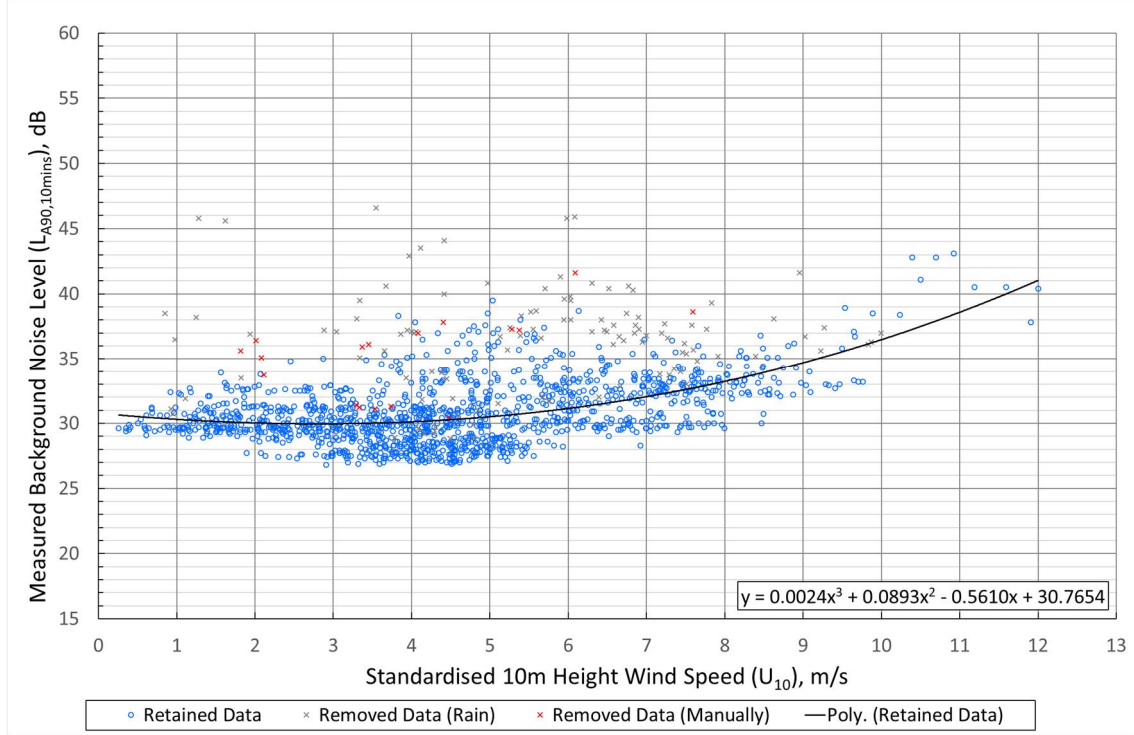
Graph 9.5.7: Location D Glenview – Quiet Daytime Background Noise (dB(A)) versus Wind Speed (m/s)
