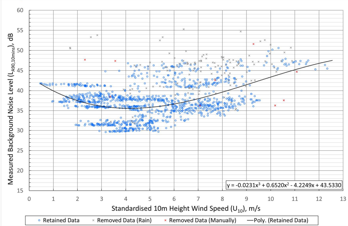
Graph 9.5.6: Location C Lamphitt – Night-time Daytime Background Noise (dB(A)) versus Wind Speed (m/s)
