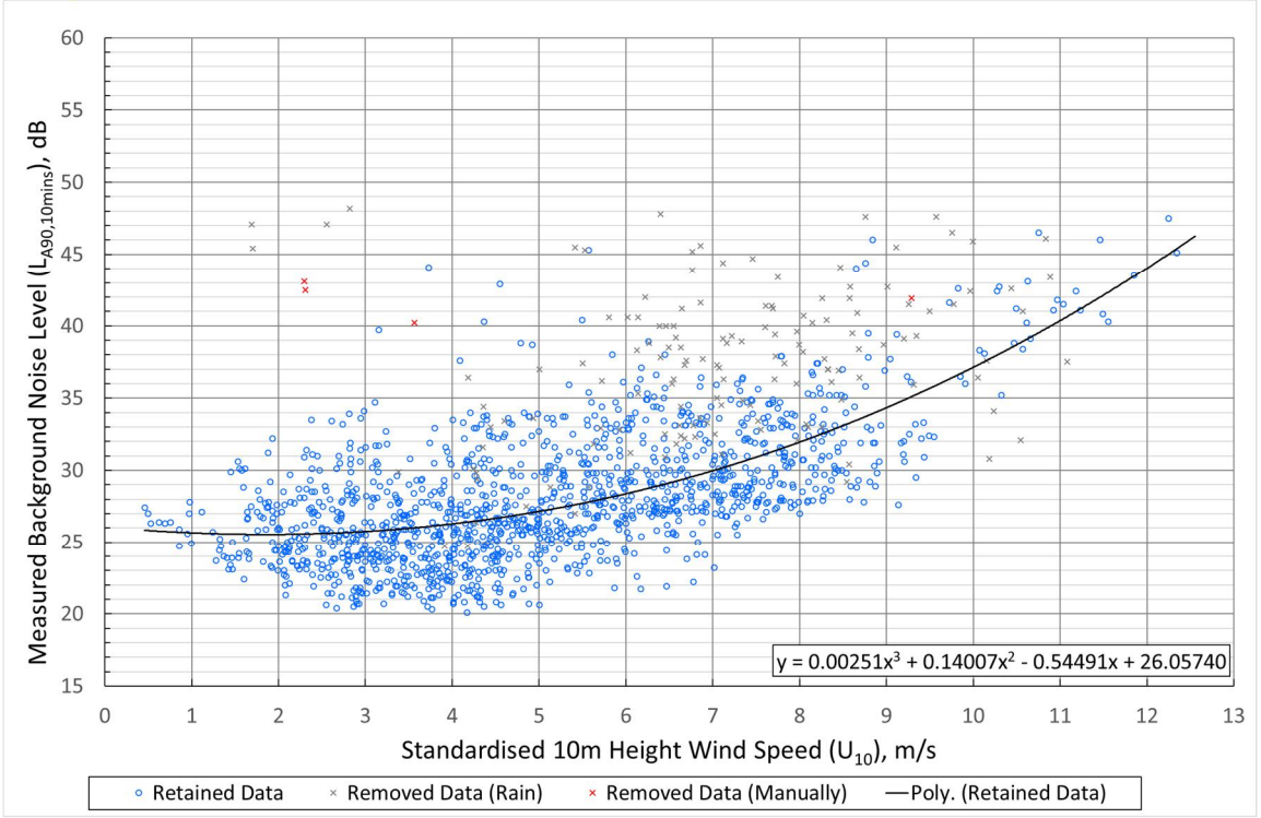
Graph 9.5.2: Location A Mollin Farm – Night-time Daytime Background Noise (dB(A)) versus Wind Speed (m/s)
