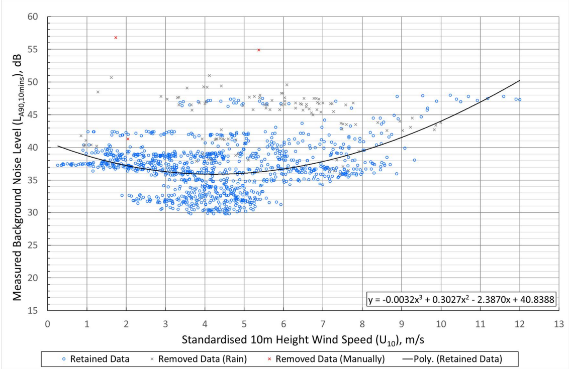
Graph 9.5.5: Location C Lamphitt – Quiet Daytime Background Noise (dB(A)) versus Wind Speed (m/s)
