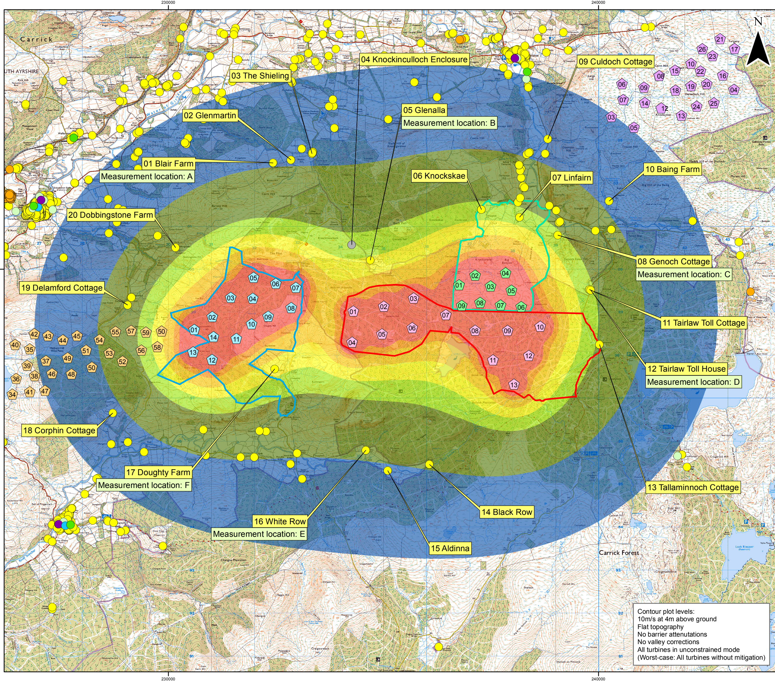
Carrick Windfarm Figure 9.4: Noise Contour - 10m/s - Proposed Developments (Carrick, Craiginmoddie and Knockcronal)
