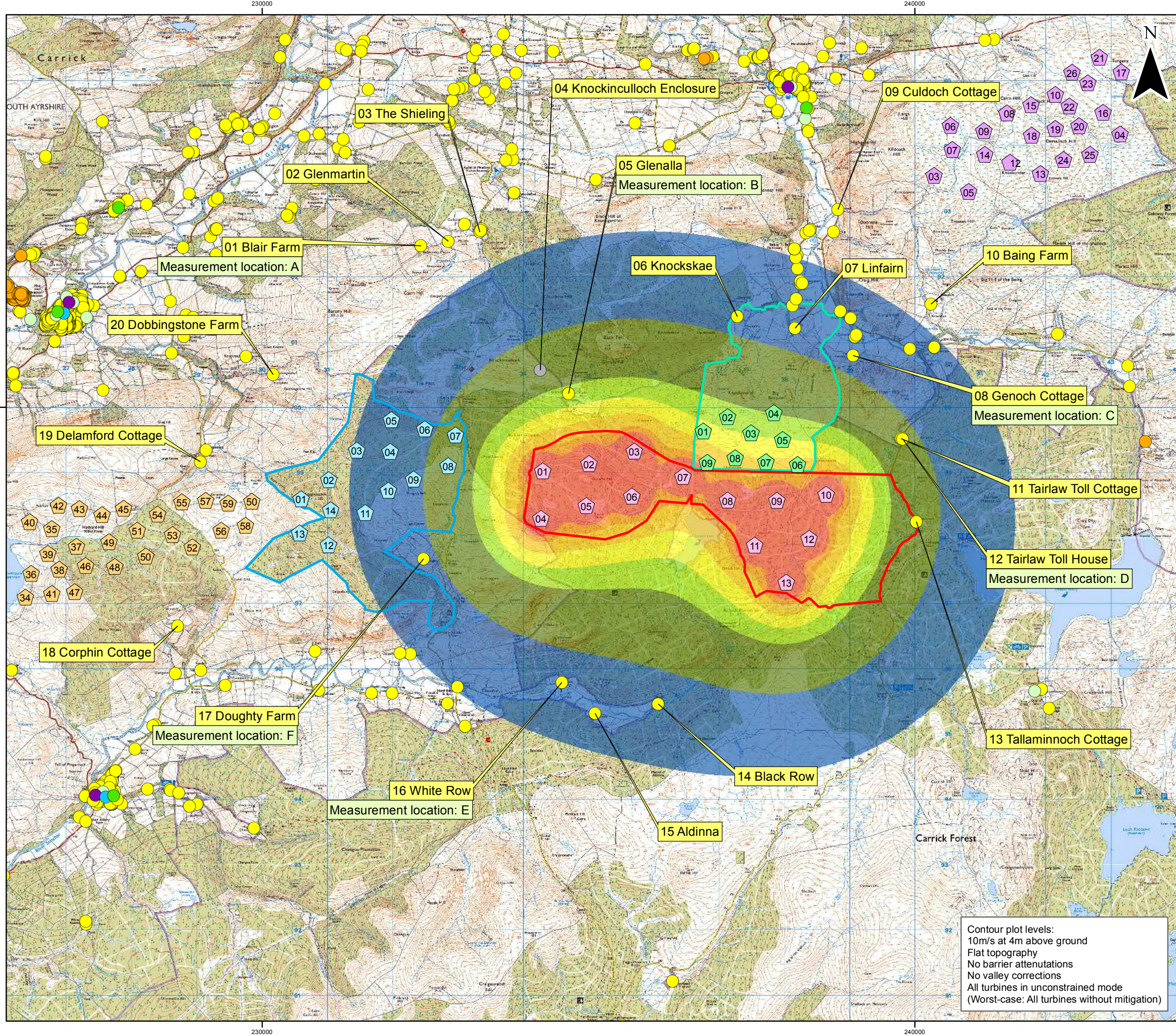
Carrick Windfarm Figure 9.2: Noise Contour- 10m/s Proposed Development (Carrick) in Isolation
