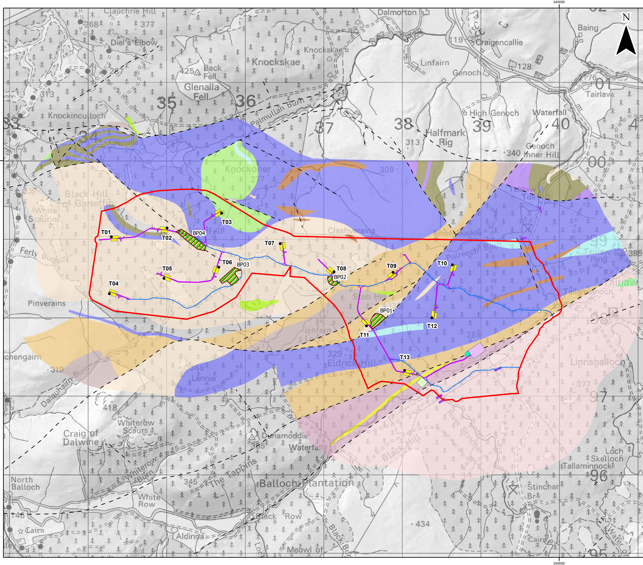
Carrick Windfarm Figure 6.2: Bedrock Geology
