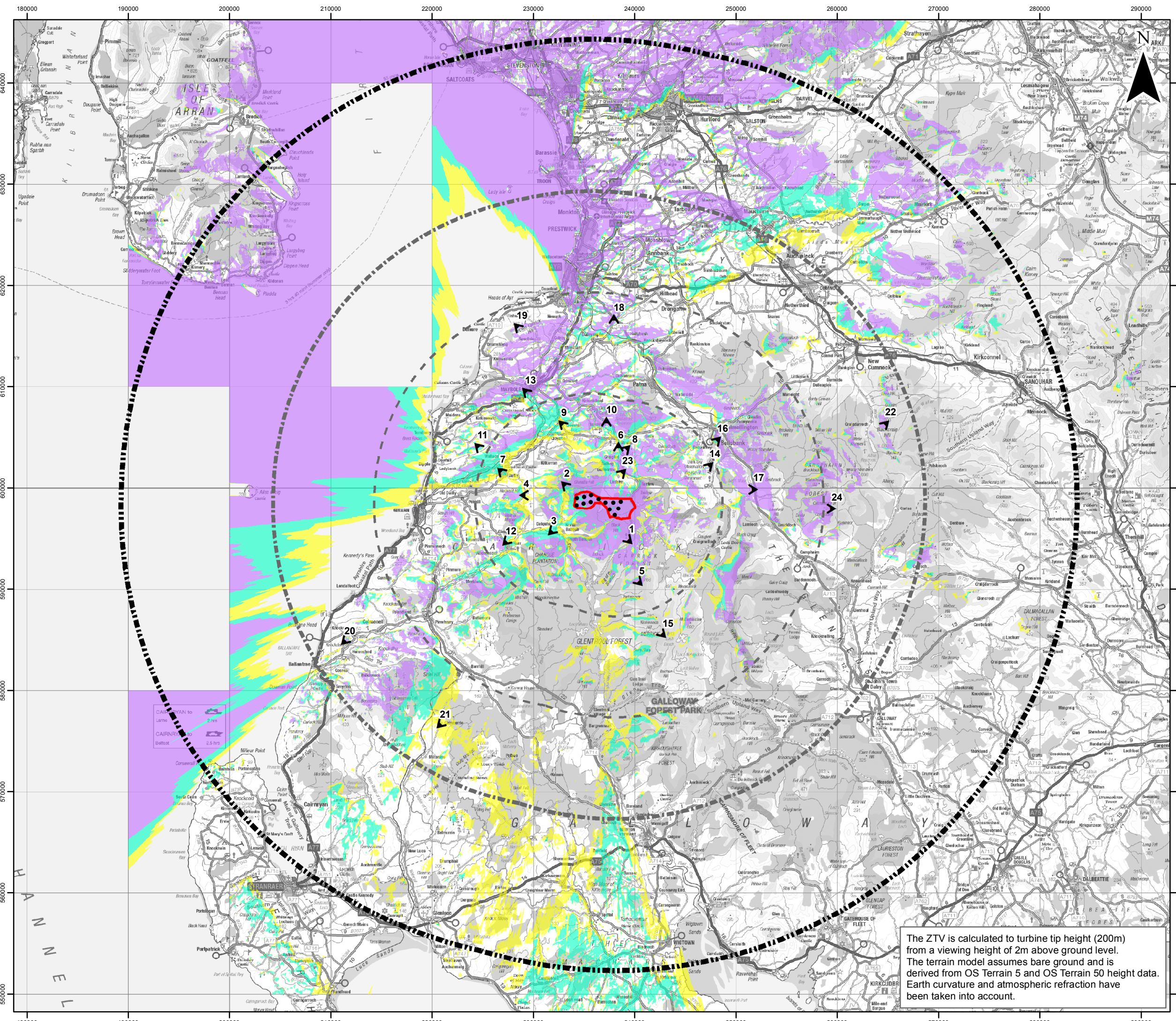
Carrick Windfarm Figure 5.2: Blade Tip ZTV - number of wind turbines visible
