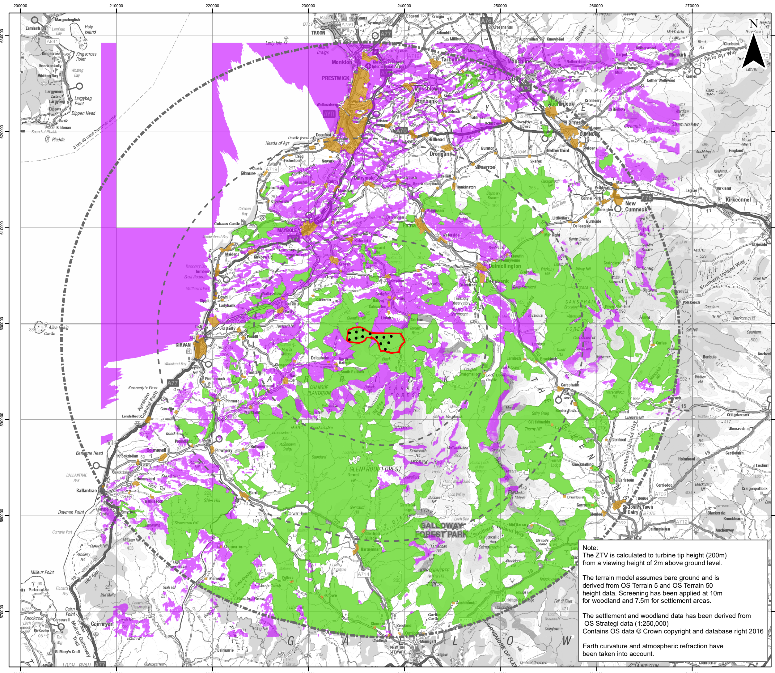
Carrick Windfarm Figure 5.1c: Blade Tip ZTV with Woodland and Settlement Screening
