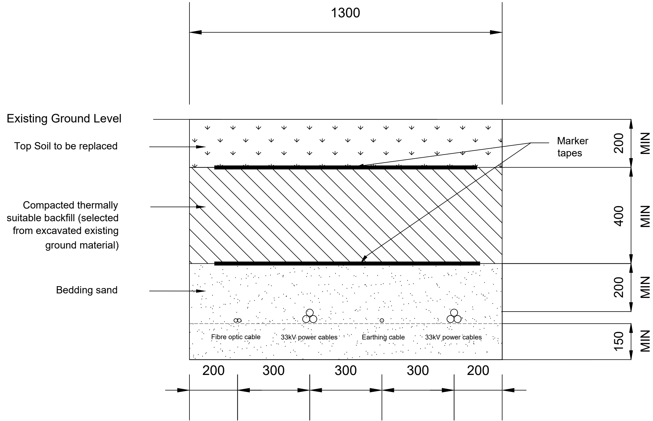
Indicative Cable Trench
