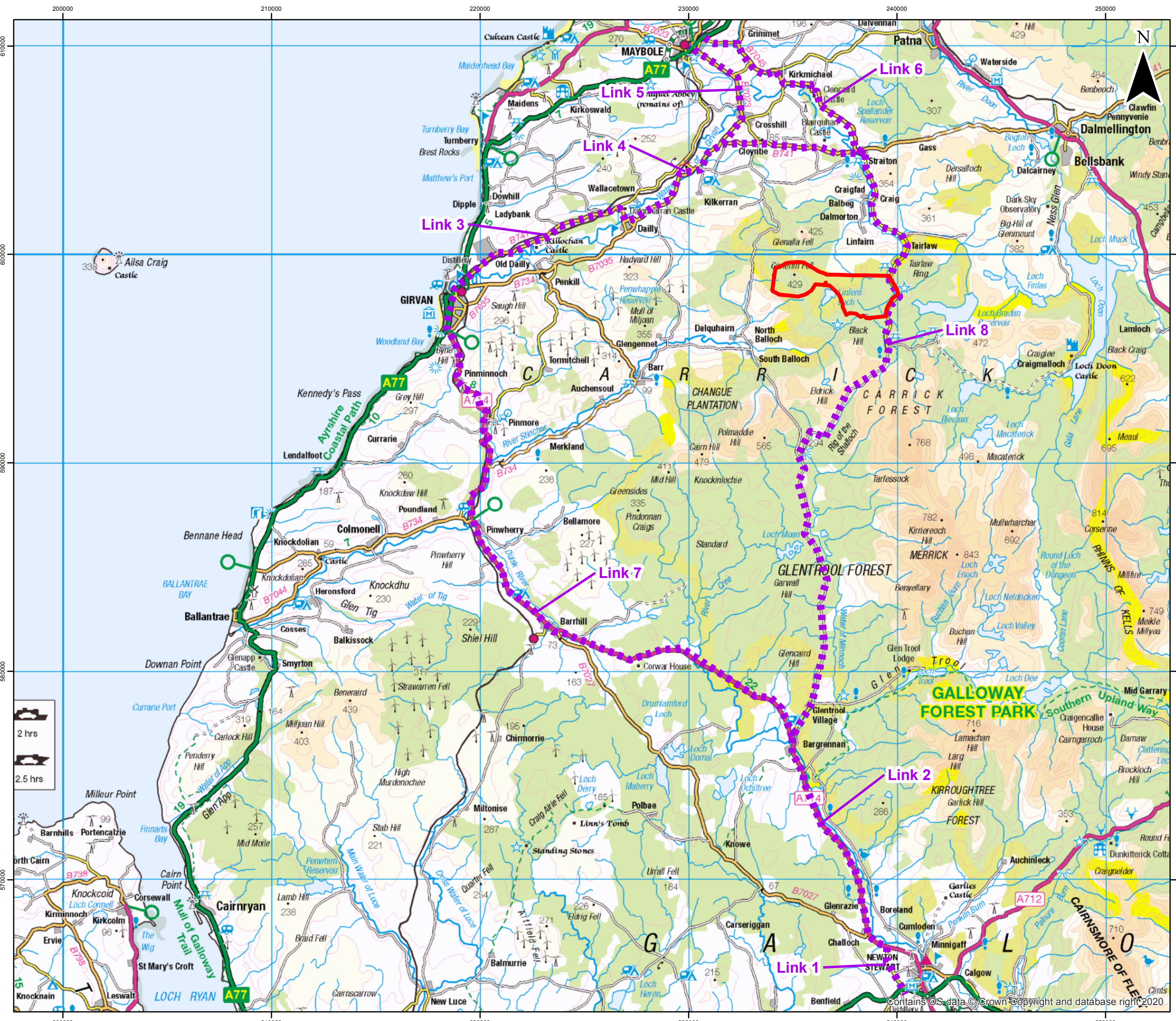
Carrick Windfarm Figure 11.2: General Construction Access Routes & Study Area Link Sections
