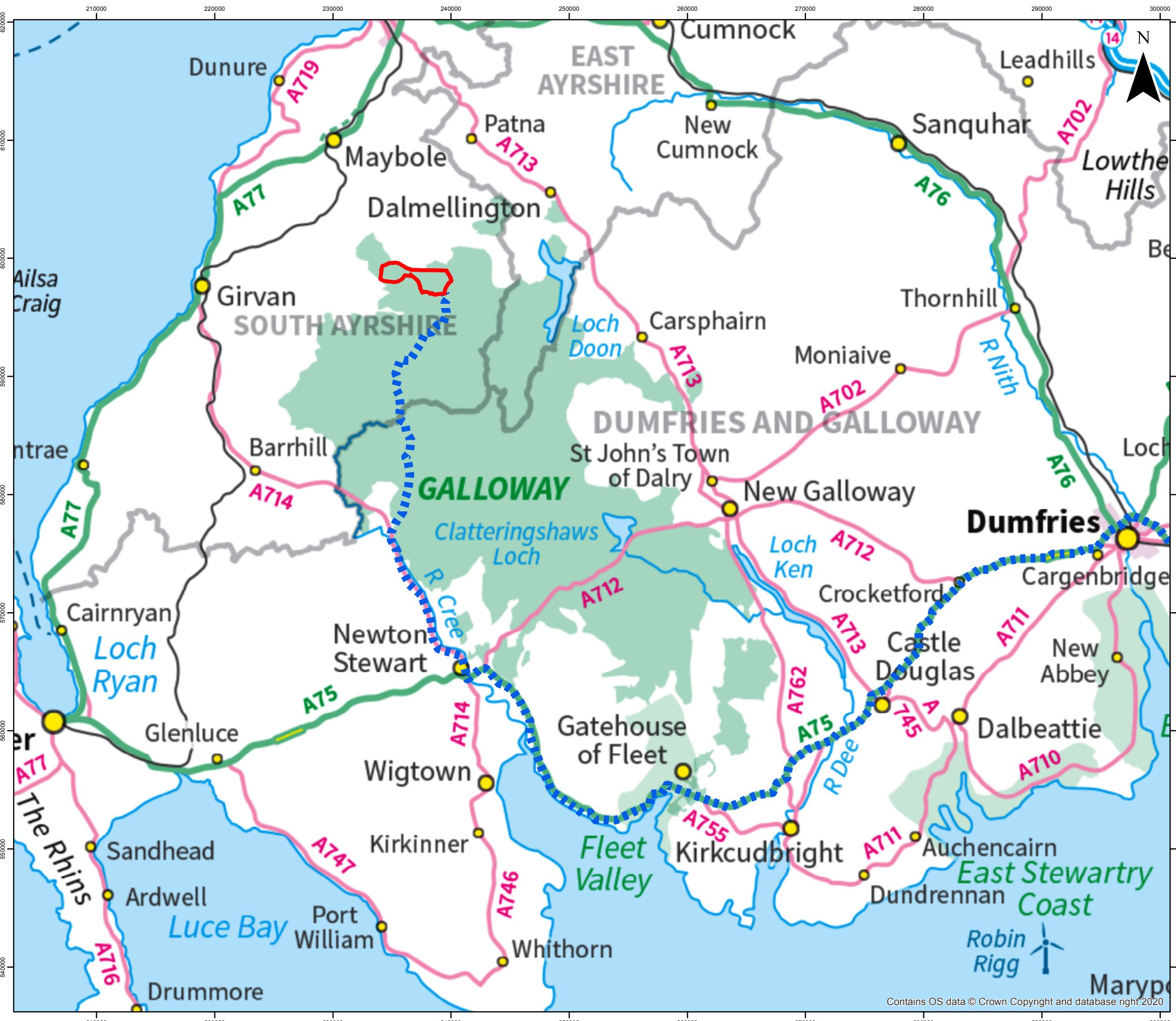
Carrick Windfarm Figure 11.1: Proposed Abnormal Load Access Route
