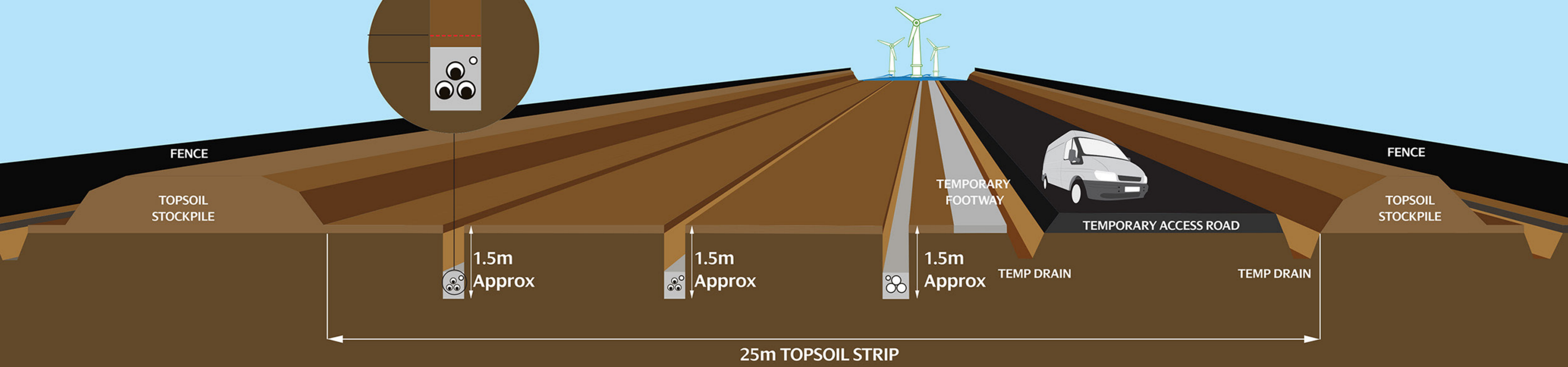
Cutaway of the onshore cable route (not to scale)
