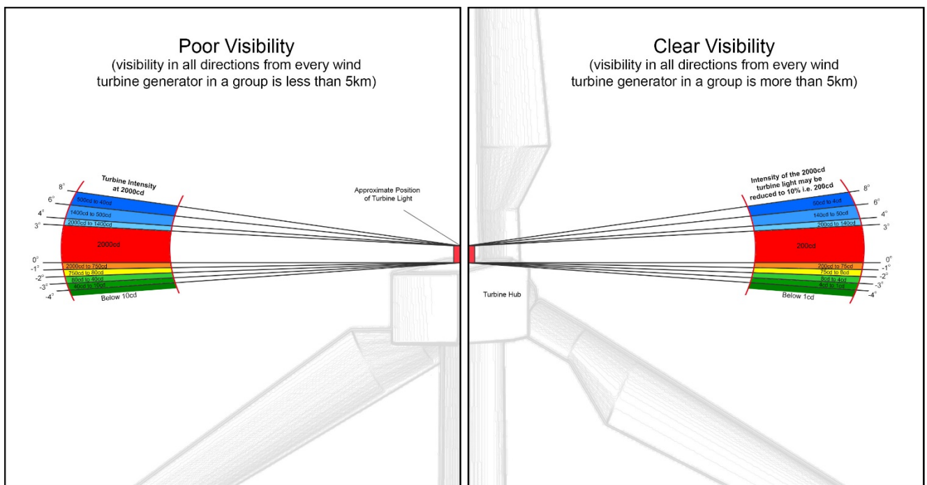
Plate TA15.3-1 Diagrammatic interpretation of minimum requirements of ICAO/CAP393 (LuxSolar Medium Intensity Obstruction Light) Note: the turbine light is designed to emit the same light intensity horizontally in 360 °.
