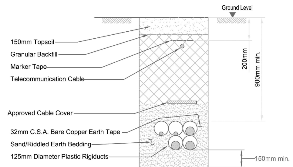
3-33kV CABLES ROAD CROSSING
