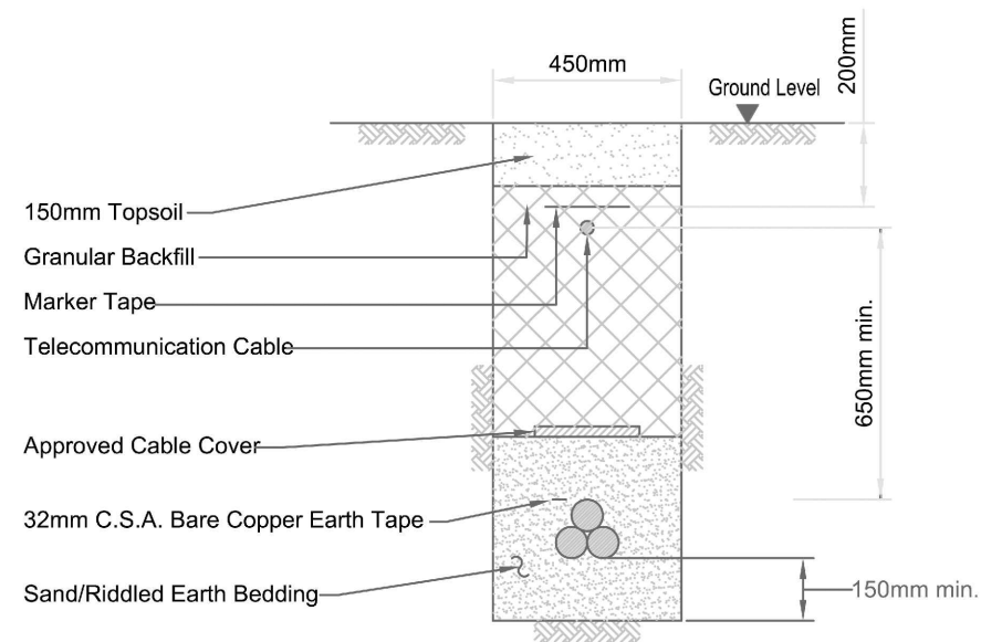
3-33kV CABLES IN TREFOIL FORMATION
