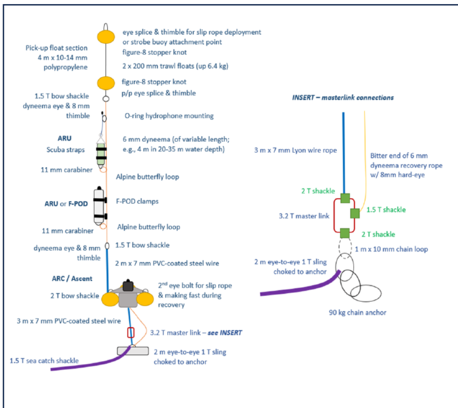
Autonomous Recording Unit (ARU)
