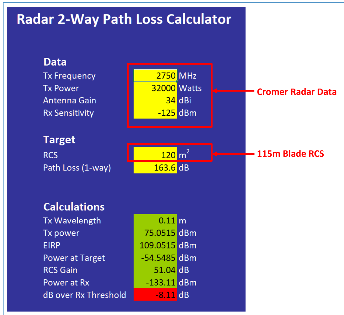
Figure 18: Cromer Radar PD Calculation for 262m Turbines
