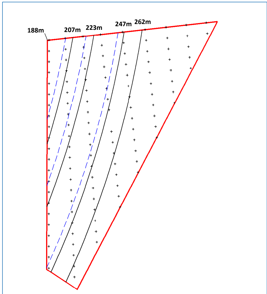
Figure 9: Trimingham Radar RLoS Contours across East Anglia THREE Site
