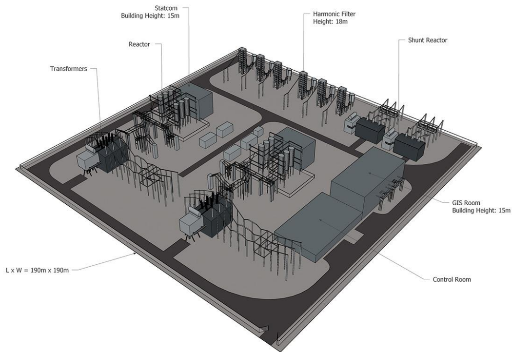
Plate A29.1 East Anglia TWO and ONE North Rochdale Envelope 3D Model
