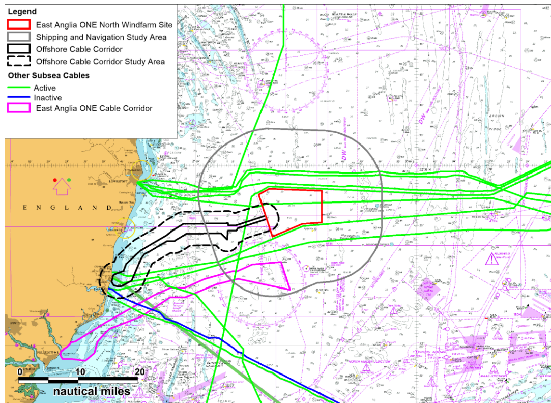
Figure 8.7 Sub-sea Cables
