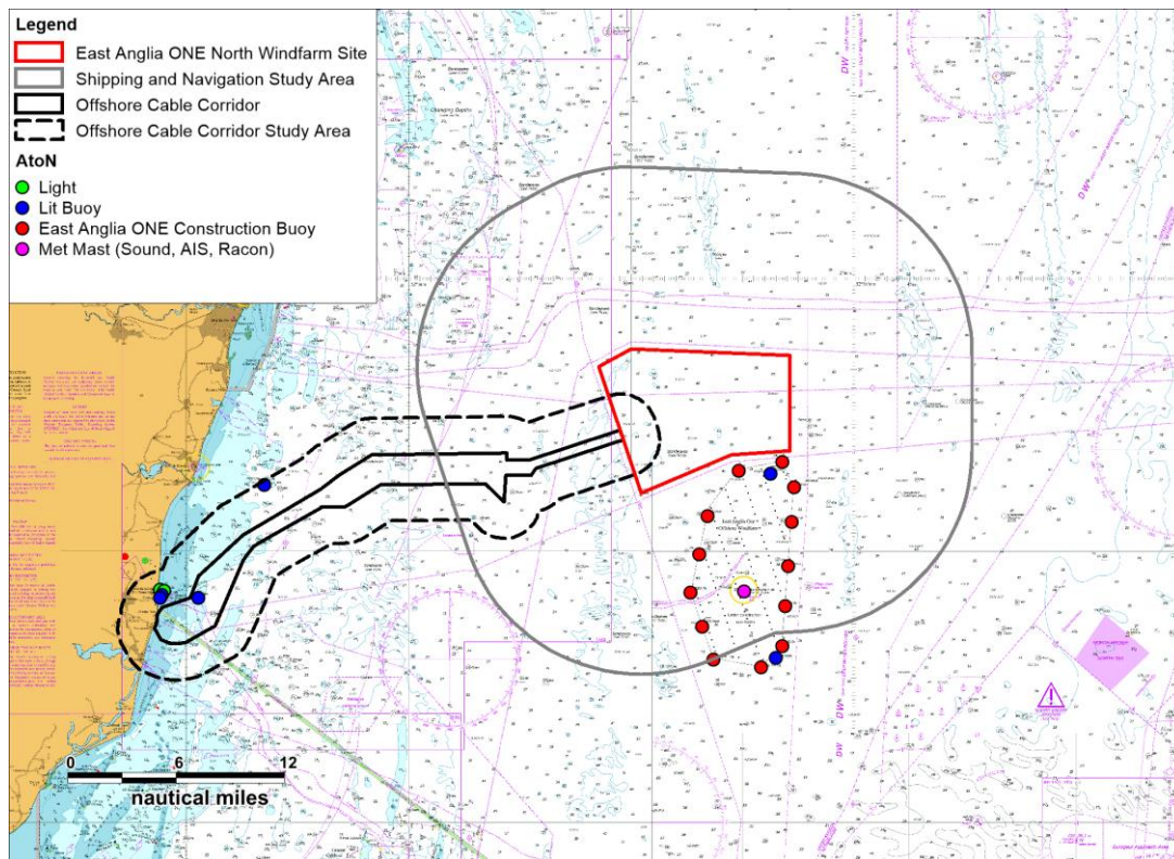
Figure 8.3 AtoN Overview
