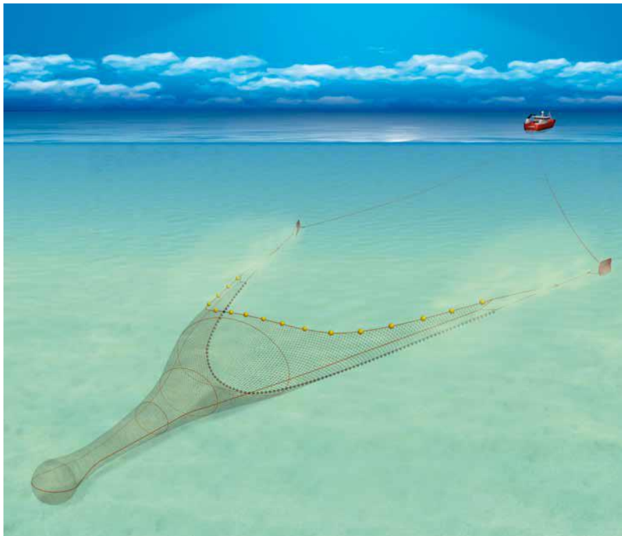
Diagram A13.1.7 Single rig otter trawl (Seafish, 2015)
