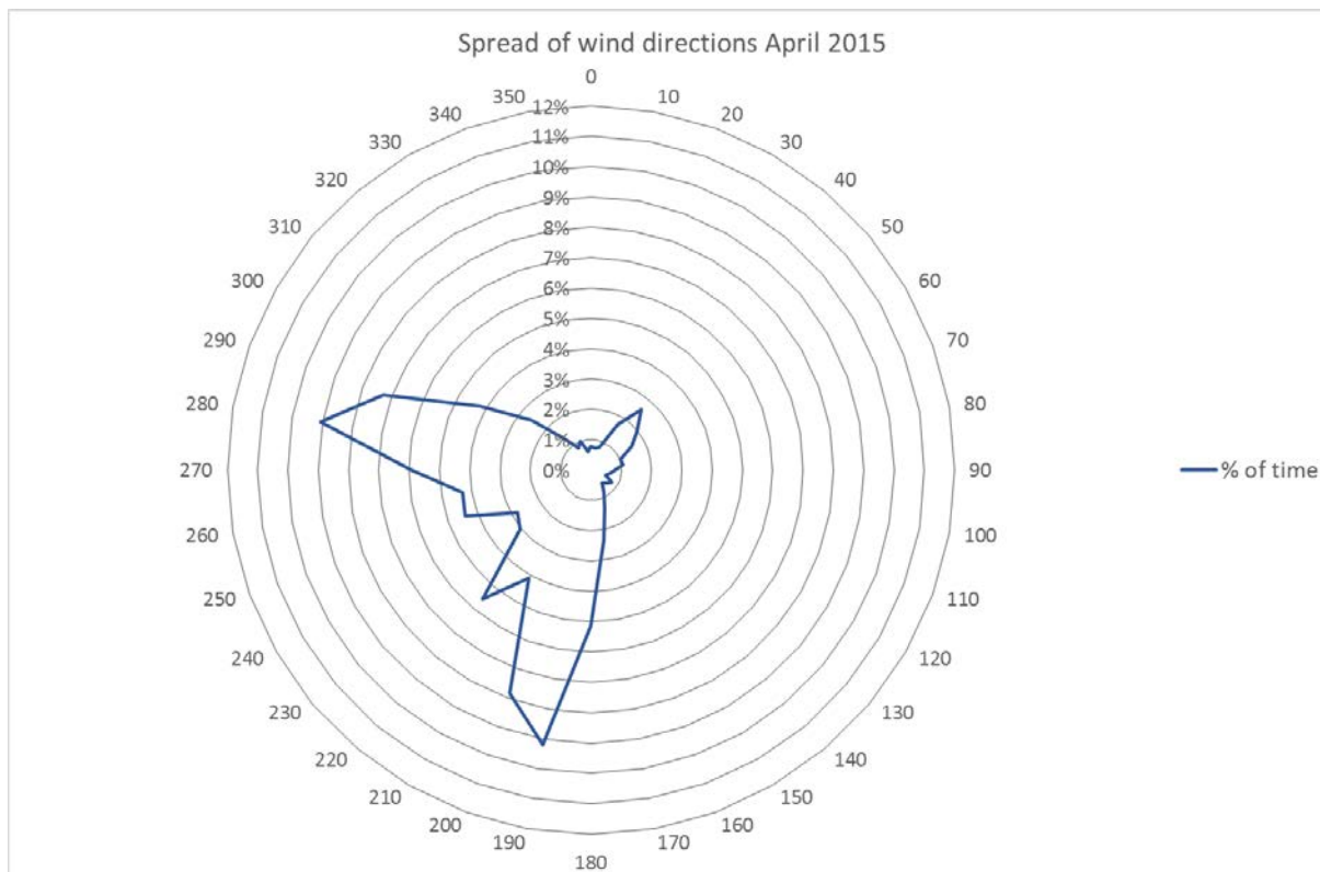
Figure 2 – Wind Rose for April 2015 Survey
