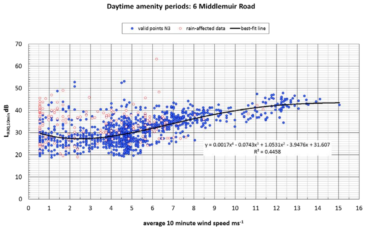
Figure 3 – Background Noise against Wind Speed at 6 Middlemuir Road
