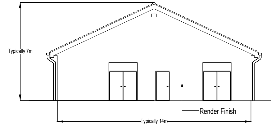
Gable End Elevation
