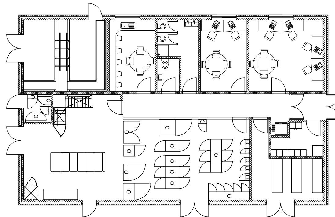
Typical Floorplan
