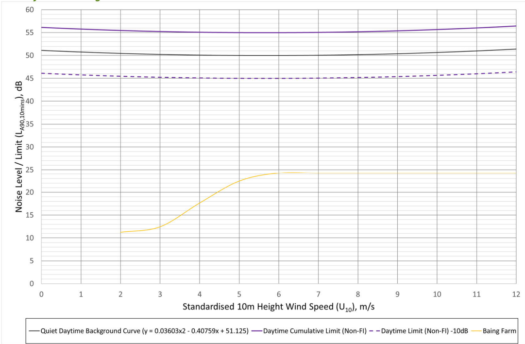
Graph 9.9.2 Baing Farm – Conditioned Dersalloch Limit -10dB Versus Proposed Development Levels
