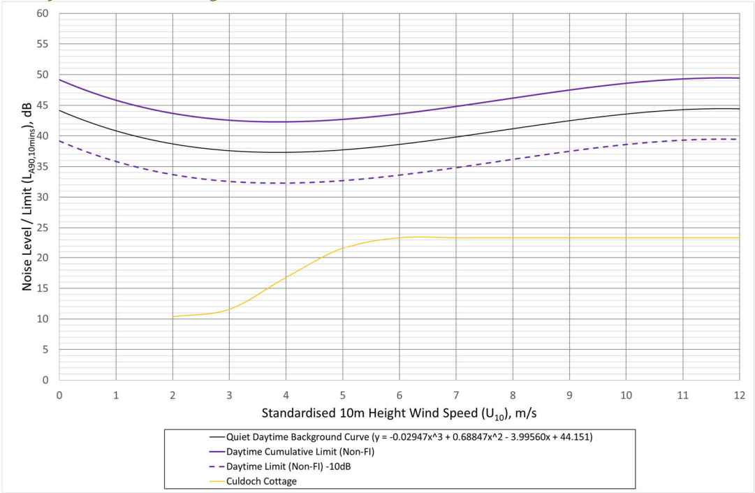
Graph 9.9.1 Culldoch Cottage – Conditioned Dersalloch Limit -10 decibels (dB) Versus Proposed Development Levels
