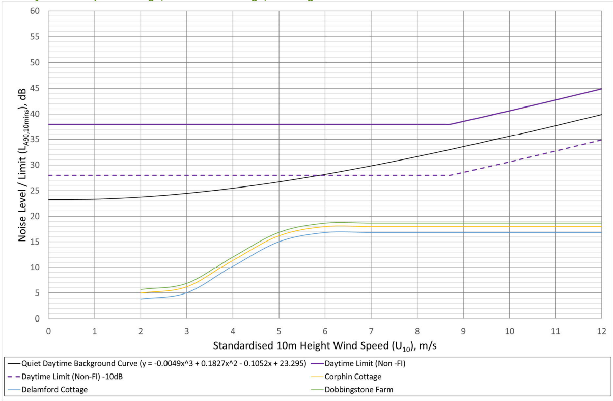
Graph 9.9.3 Corphin Cottage, Delamford Cottage, Dobbingsstone Farm - Determined Cumulative Limit -10dB Versus Proposed Development Levels
