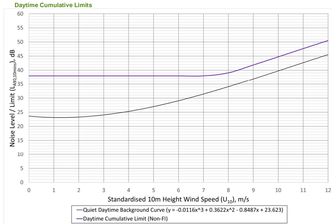
Graph 9.7.1 Location A Blair Farm – Daytime Cumulative Noise Limit, dB(A) Versus Wind Speed (m/s)
