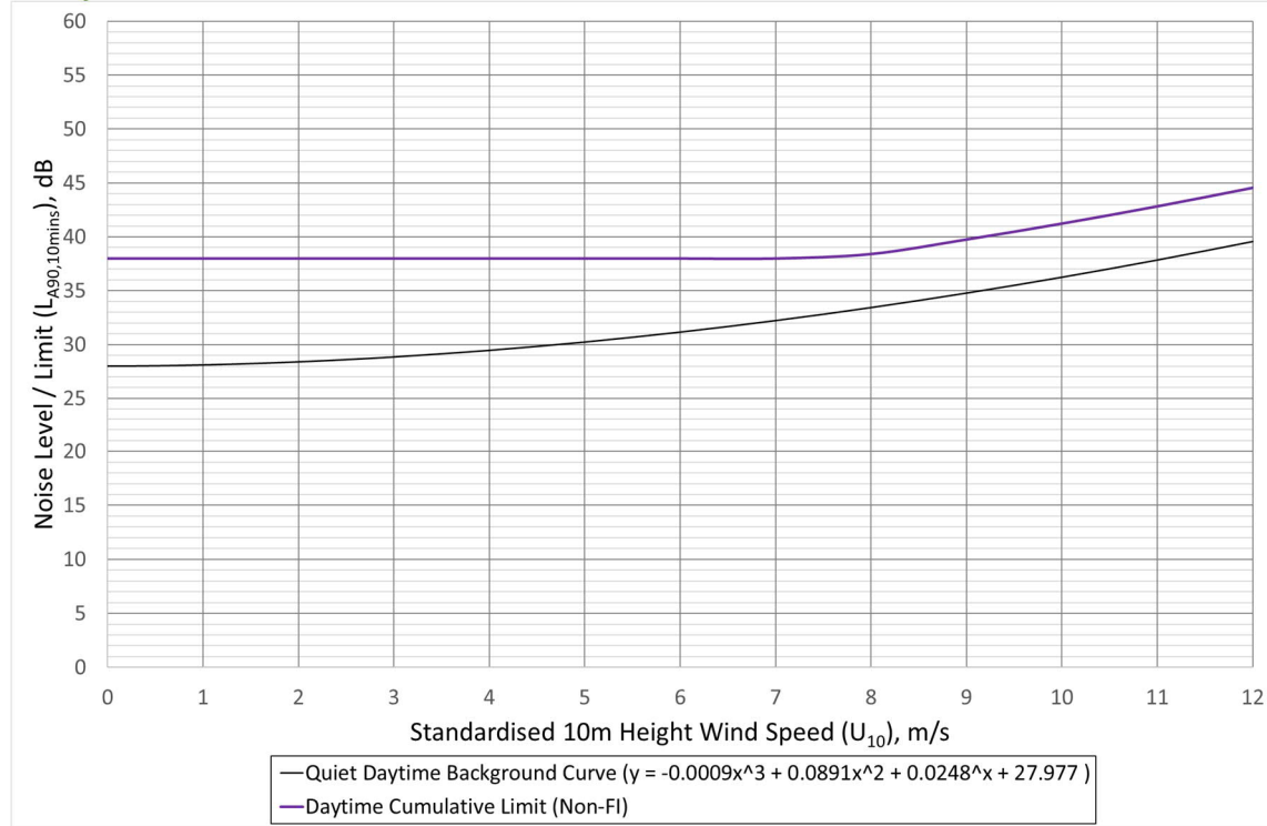
Graph 9.7.5 Location C Genoch Cottage – Daytime Cumulative Noise Limit, dB(A) Versus Wind Speed (m/s)
