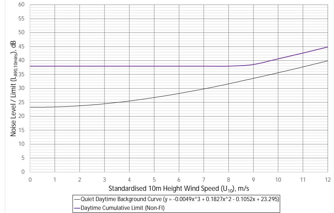
Graph 9.7.11 Location F Doughty Farm – Daytime Cumulative Noise Limit, dB(A) Versus Wind Speed (m/s)
