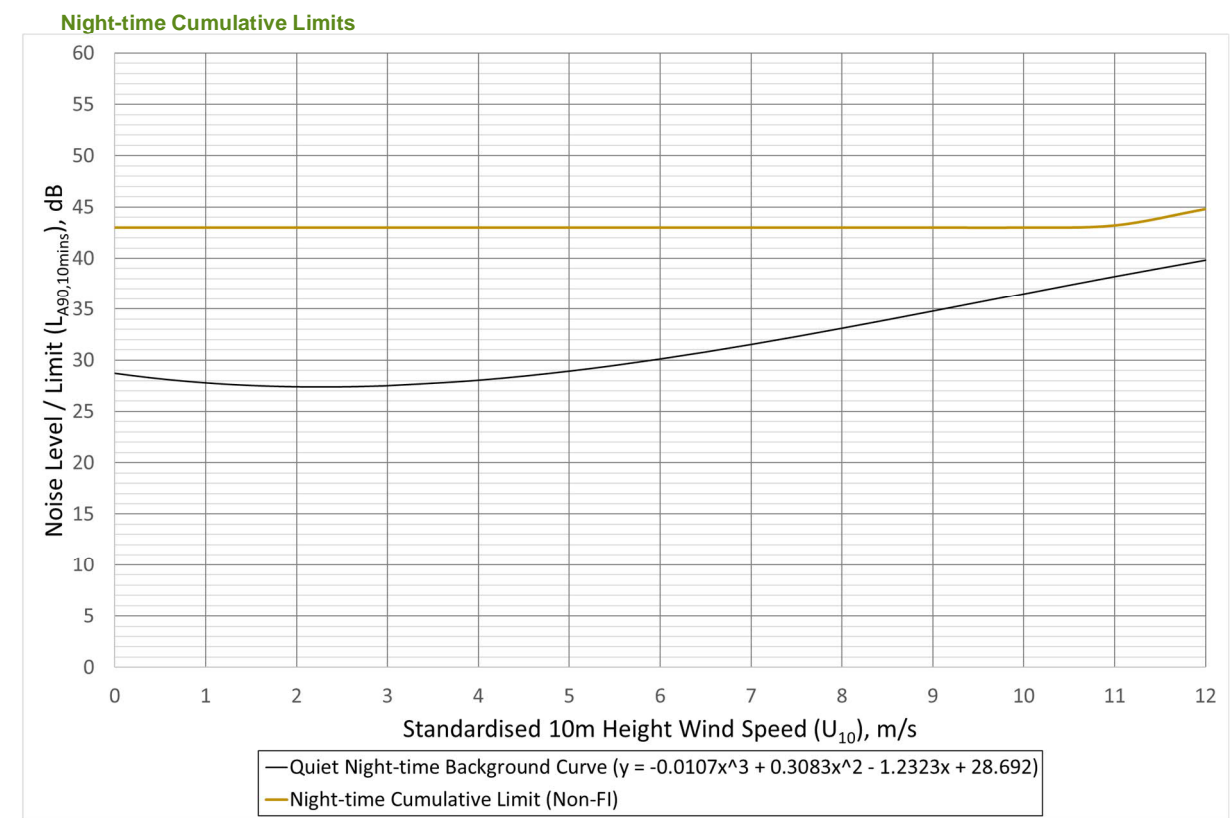
Graph 9.7.4 Location B Glenalla – Night-time Cumulative Noise Limit, dB(A) Versus Wind Speed (m/s)
