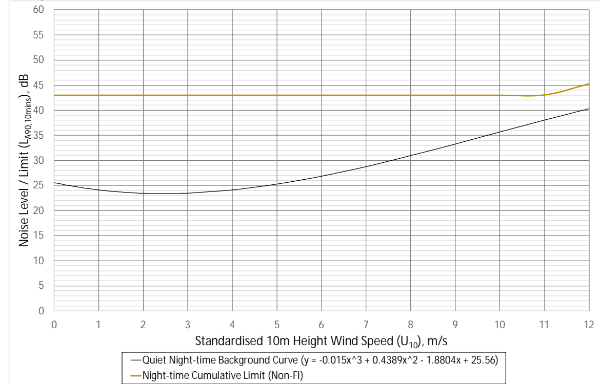
Graph 9.7.12 Location D Doughty Farm – Night-time Cumulative Noise Limit, dB(A) Versus Wind Speed (m/s)
