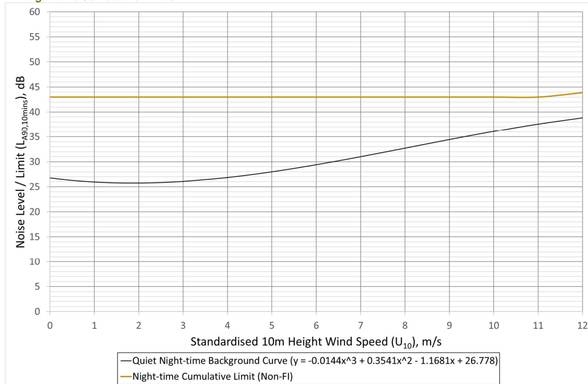
Graph 9.7.6 Location C Genoch Cottage – Night-time Cumulative Noise Limit, dB(A) Versus Wind Speed (m/s)
