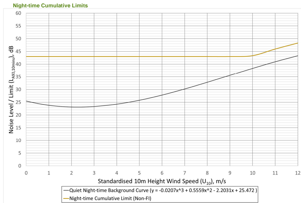
Graph 9.7.2 Location A Blair Farm – Night-time Cumulative Noise Limit, dB(A) Versus Wind Speed (m/s)
