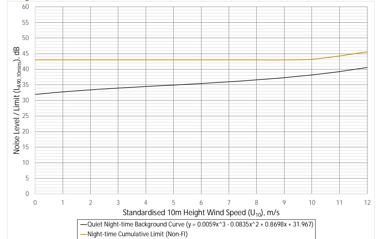
Graph 9.7.8 Location D Tairlaw Toll – Night-time Cumulative Noise Limit, dB(A) Versus Wind Speed (m/s)
