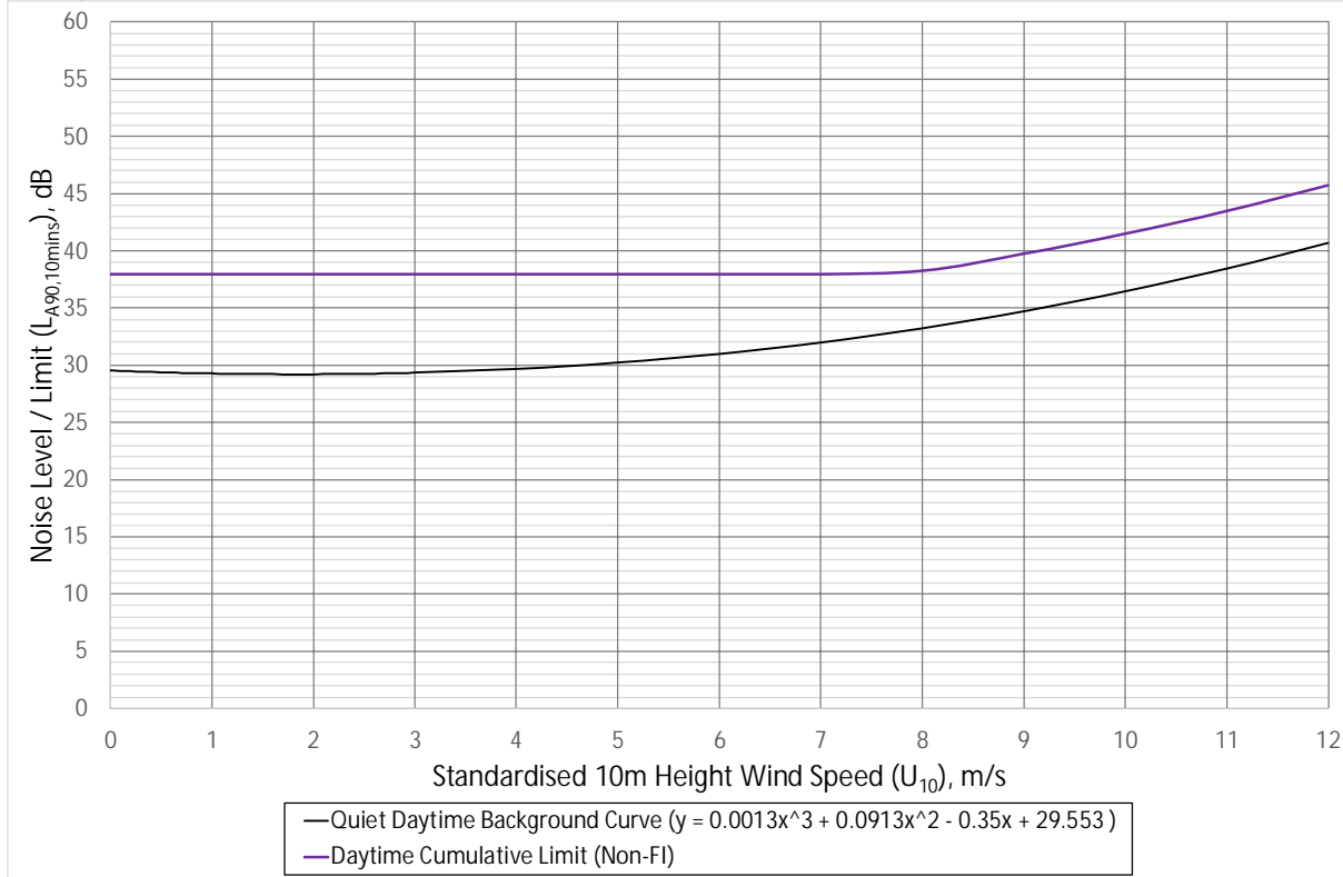
Graph 9.7.9 Location E White Row – Daytime Cumulative Noise Limit, dB(A) Versus Wind Speed (m/s)
