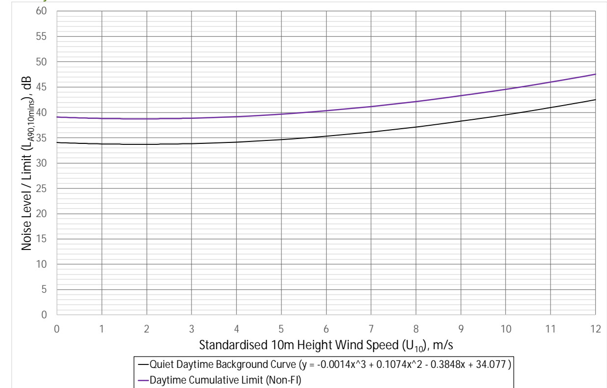
Graph 9.7.7 Location D Tairlaw Toll – Daytime Cumulative Noise Limit, dB(A) Versus Wind Speed (m/s)
