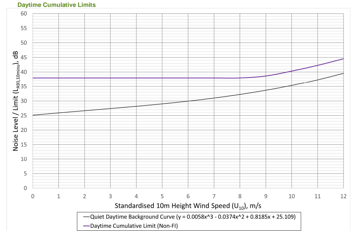
Graph 9.7.3 Location B Glenalla – Daytime Cumulative Noise Limit, dB(A) Versus Wind Speed (m/s)
