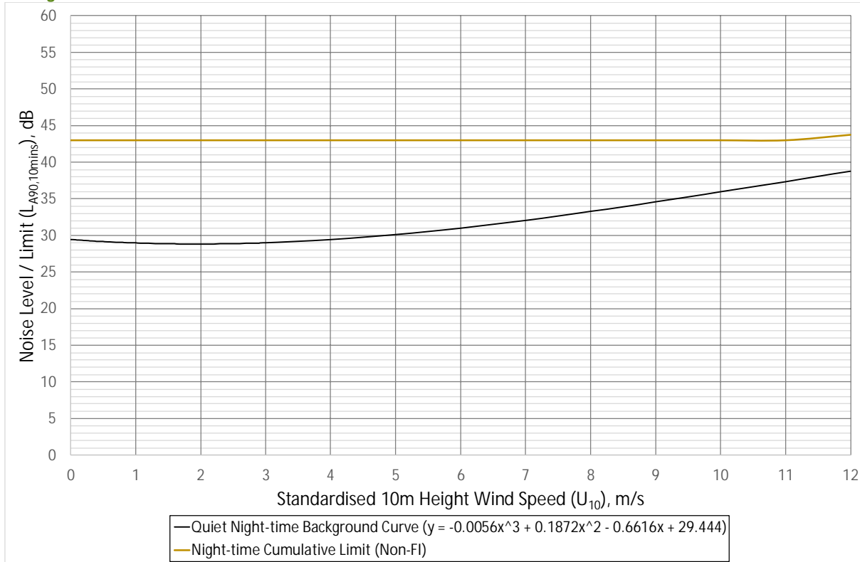
Graph 9.7.10 Location E White Row – Night-time Cumulative Noise Limit, dB(A) Versus Wind Speed (m/s)
