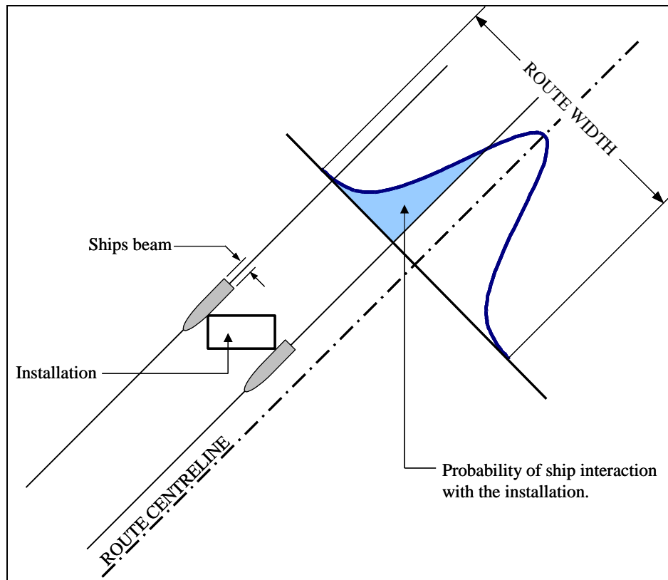
Figure 3.1 Geometrical Probability of a Collision Course
