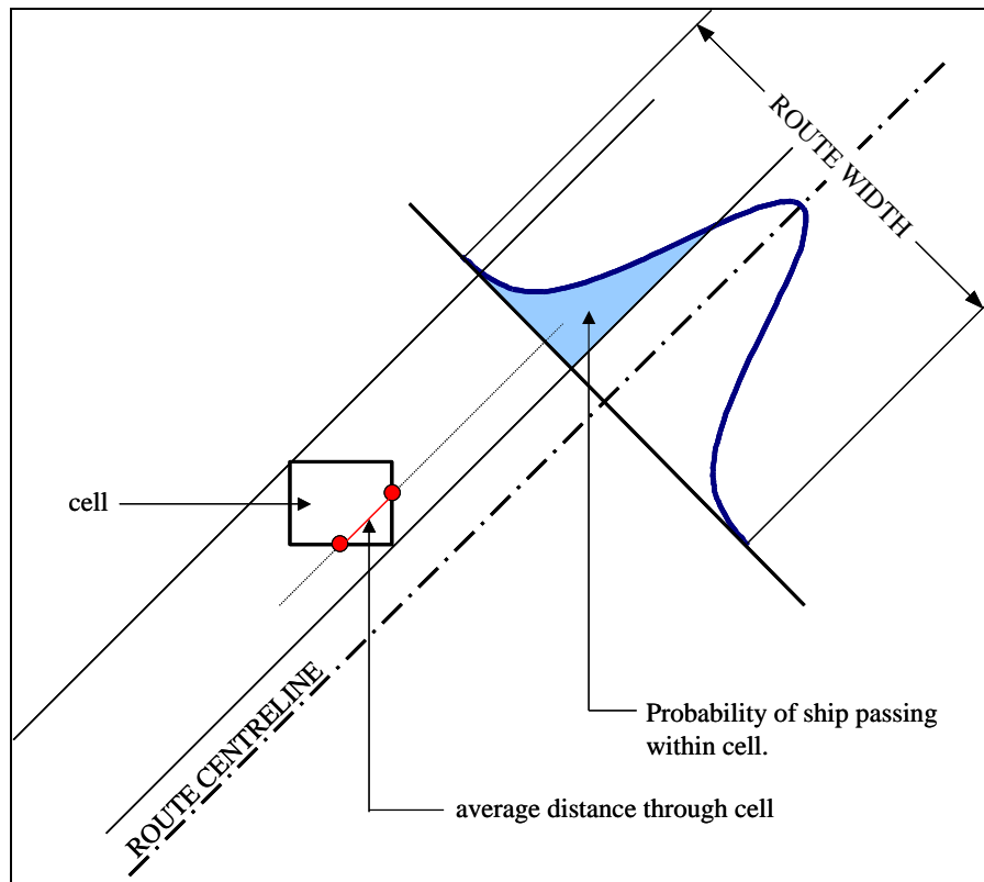
Figure 2.1 Calculation of Distance Travelled by Ships within a Cell
