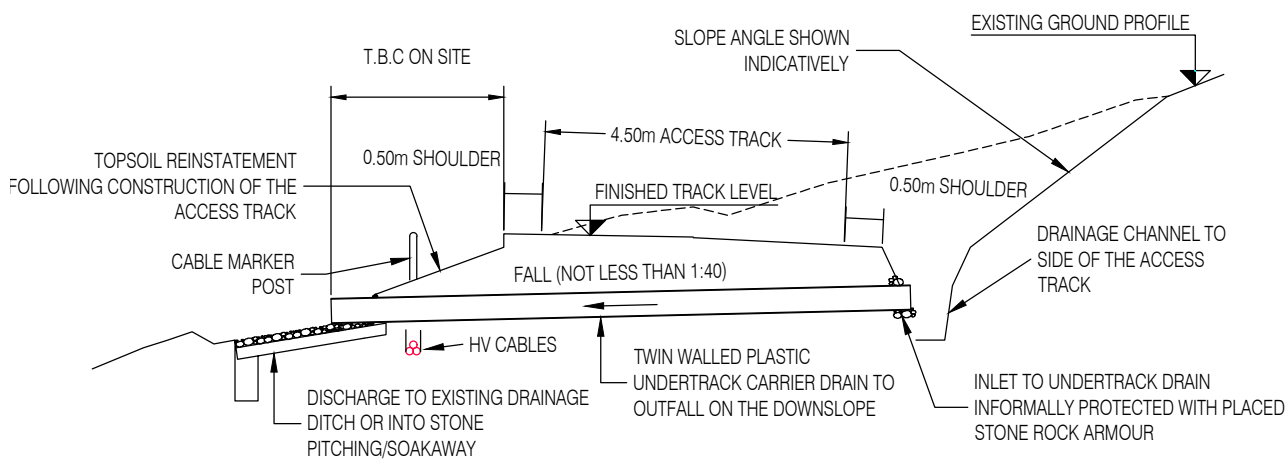
TYPICAL CROSS SECTION 'A-A' THROUGH TRACK ON SIDE OF SLOPE SCALE 1:100
