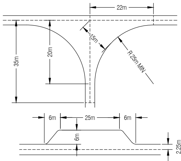
TYPICAL PASSING PLACES/TURNING HEADS N.T.S.
