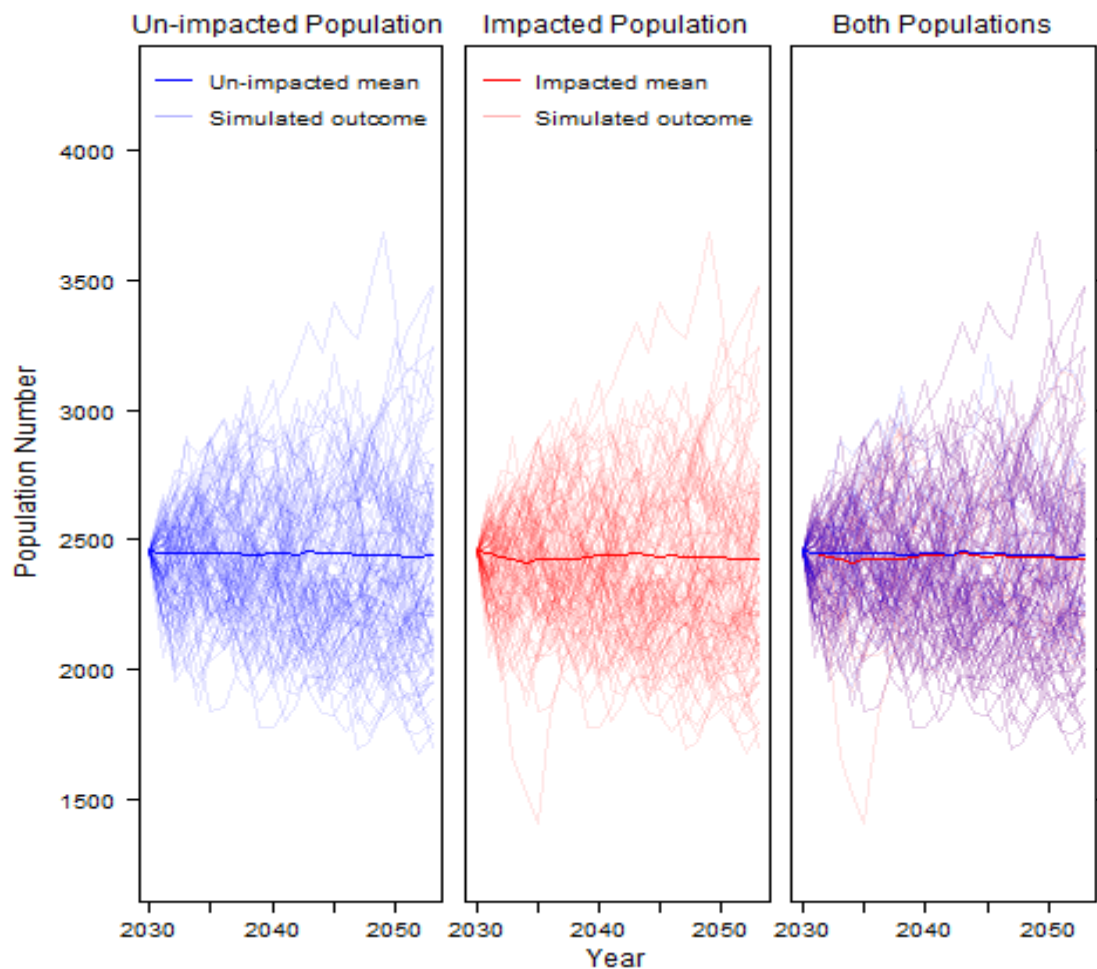
Plate 6.1 Simulated worst-case minke whale WS population sizes for both the unimpacted and the impacted populations using disturbance only
