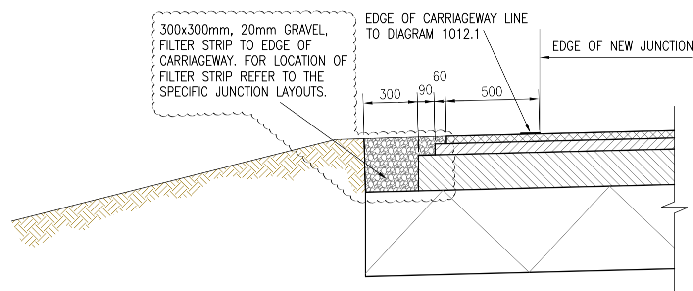
CROSS SECTION THROUGH EDGE OF NEW ACCESS CONSTRUCTION SCALE 1:20
