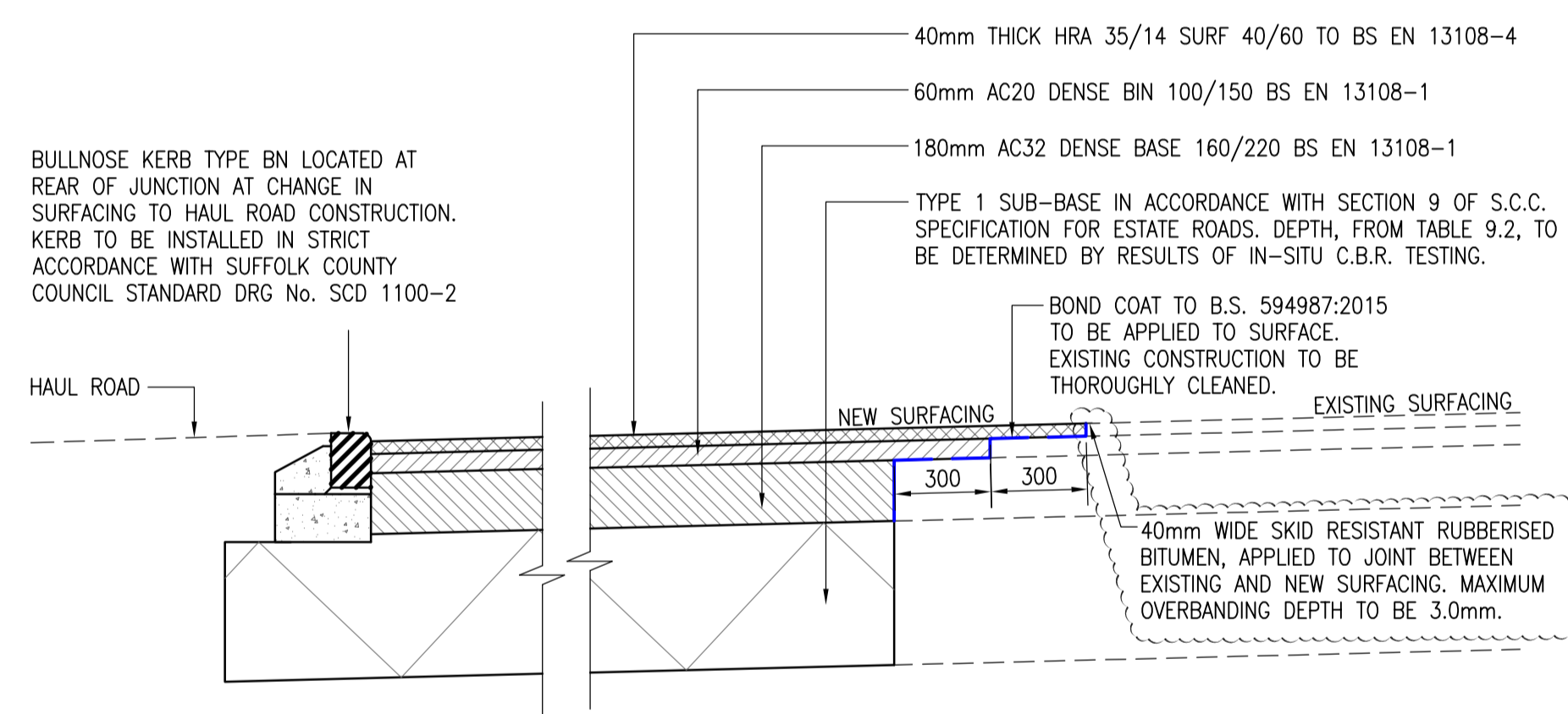
SECTION THROUGH NEW ACCESS CONSTRUCTION AT TIE-IN TO EXISTING CARRIAGEWAY SCALE 1:20
