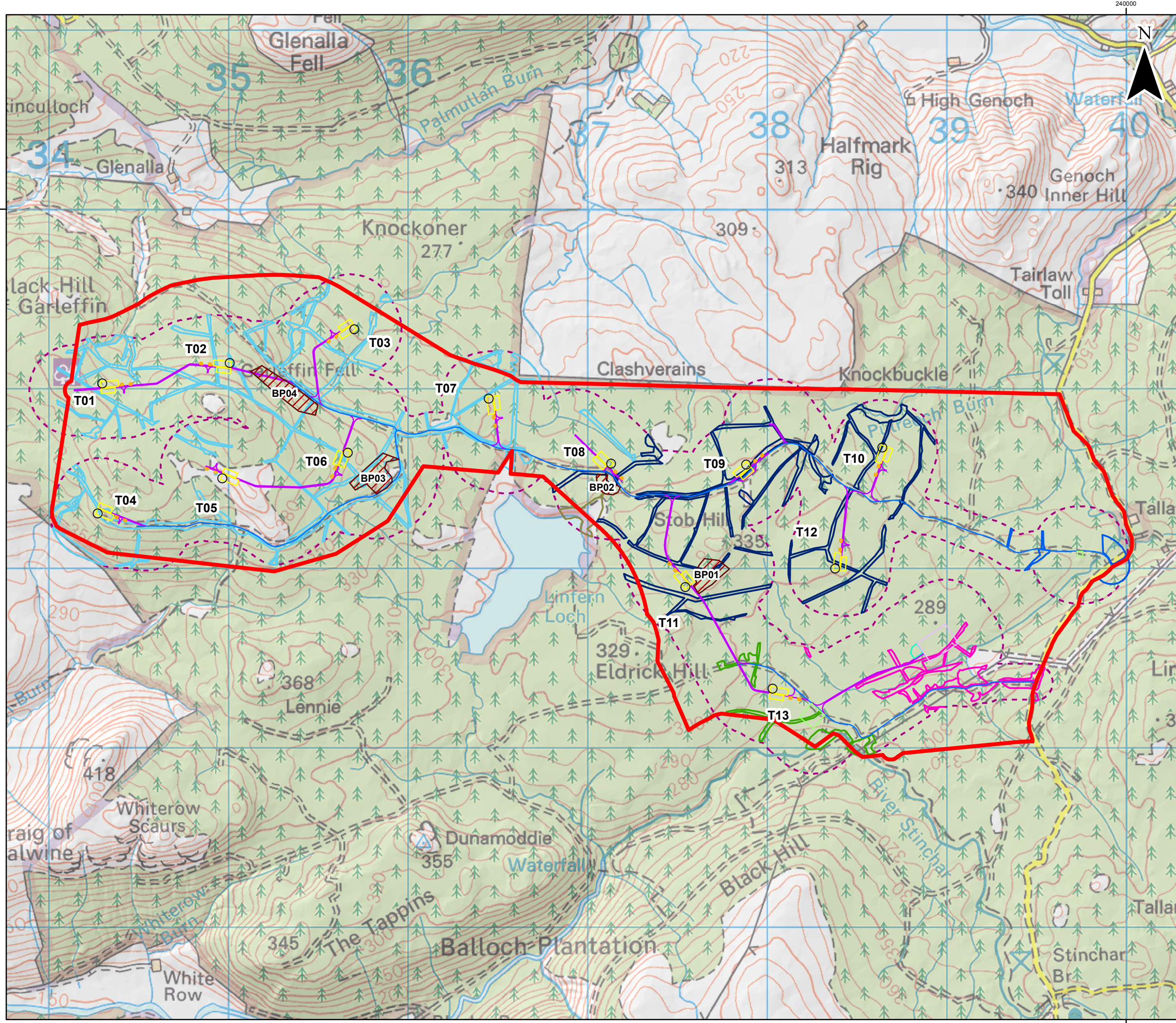
Carrick Windfarm Figure 6.6a: Groundwater Dependent Terrestrial Ecosystems Overview (Cluster Groupings)
