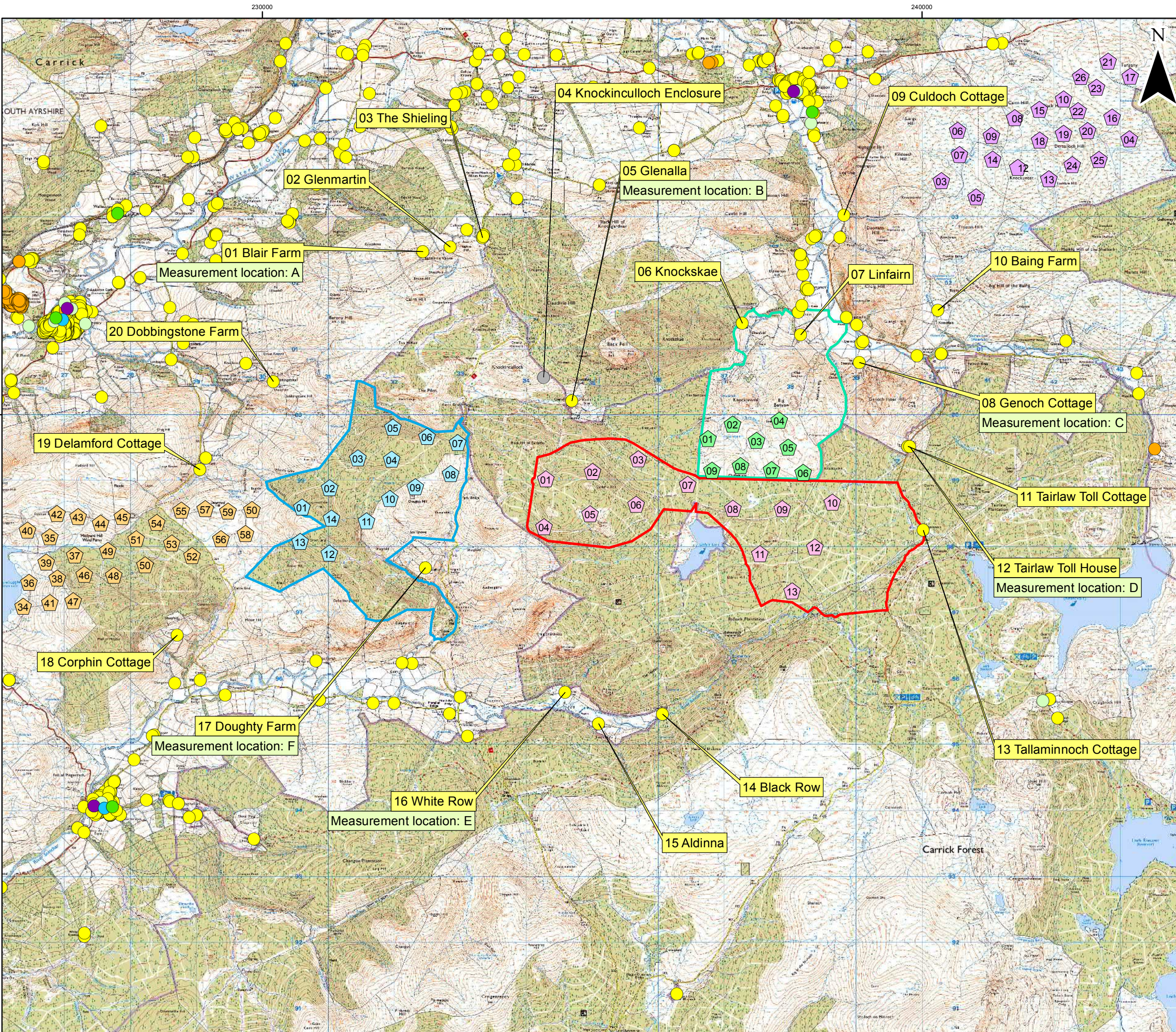
Carrick Windfarm Figure 9.1: Noise and Vibration Sensitive Receptors, Cumulative Developments and Baseline Noise Measurement Locations
