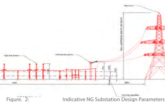
Figure. 2: Indicative NG Substation Design Parameters
