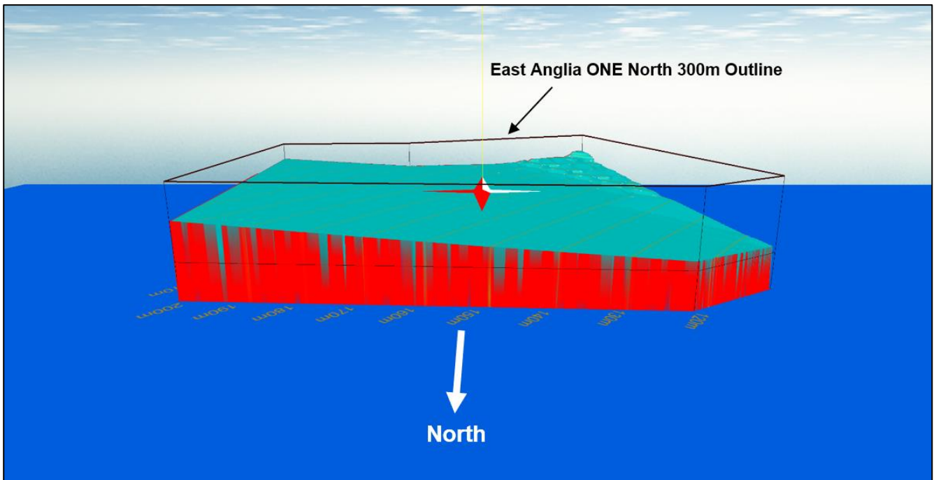
DiagramA15.1.11 3D representation of Trimmingham PSR RLoS to East Anglia ONE North, viewed from the north
