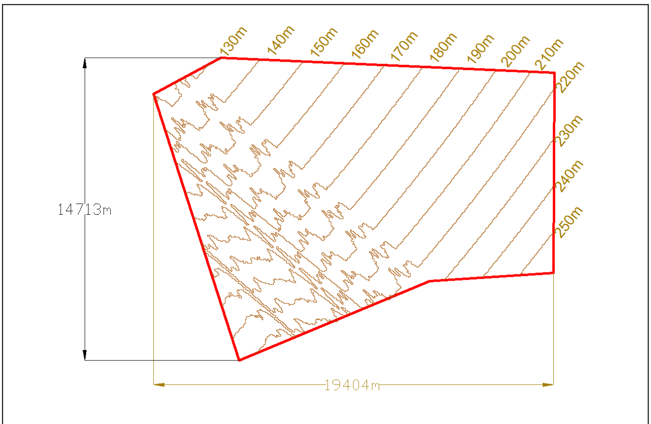
DiagramA15.1.23 Cromer radar RLoS to East Anglia ONE North
