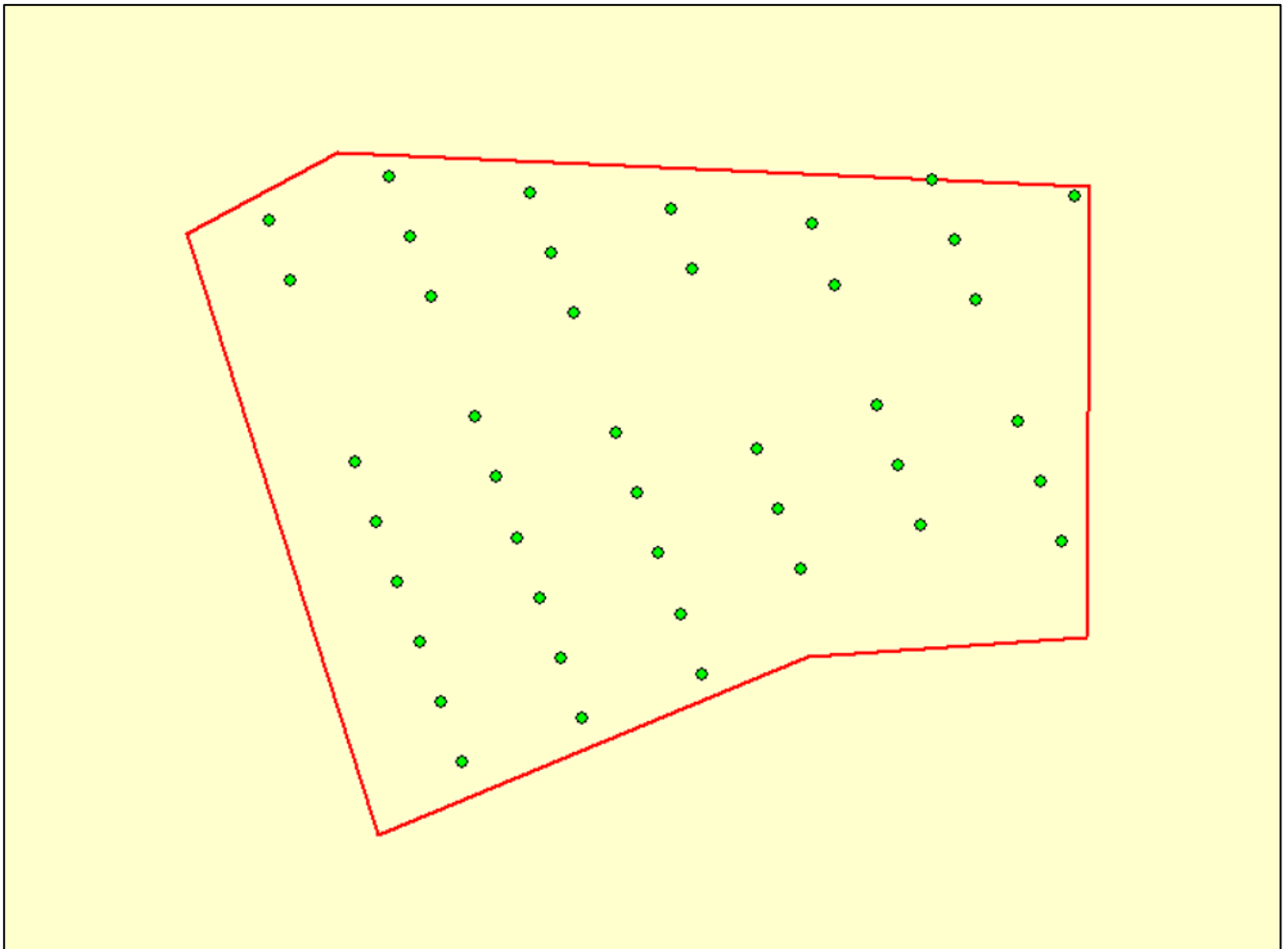
DiagramA15.1.3 Max Tip 300m Turbine Indicative Layout – 42 Turbines
