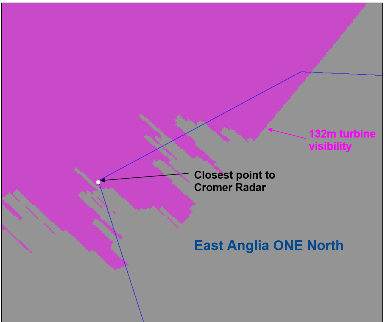
DiagramA15.1.28 Cromer radar visibility to 132m turbine – East Anglia ONE North
