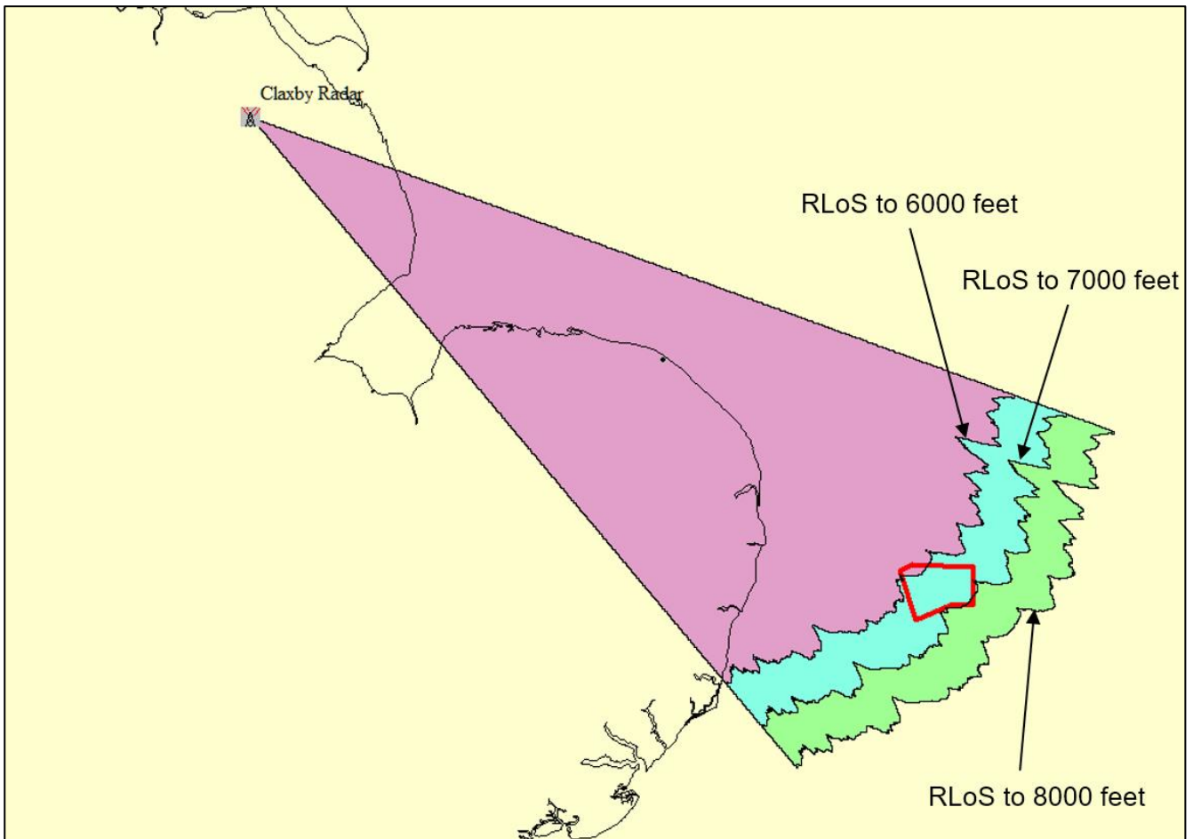
DiagramA15.1.36 Claxby radar RLoS coverage to 6000 feet, 7000 feet and 8000 feet
