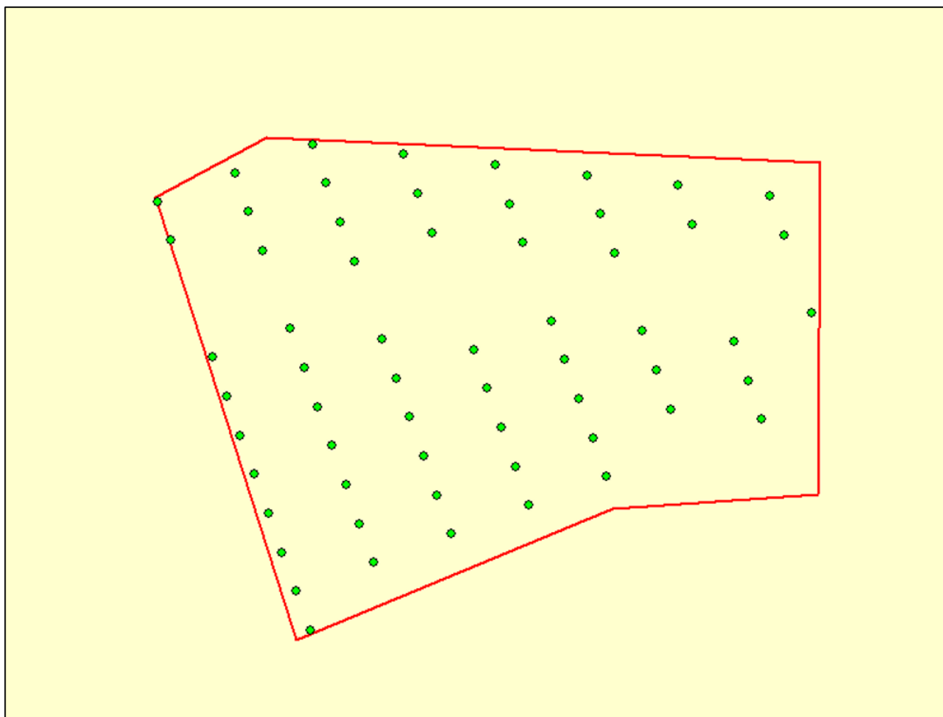
DiagramA15.1.2 Max Tip 244m Turbine Indicative Layout – 60 Turbines
