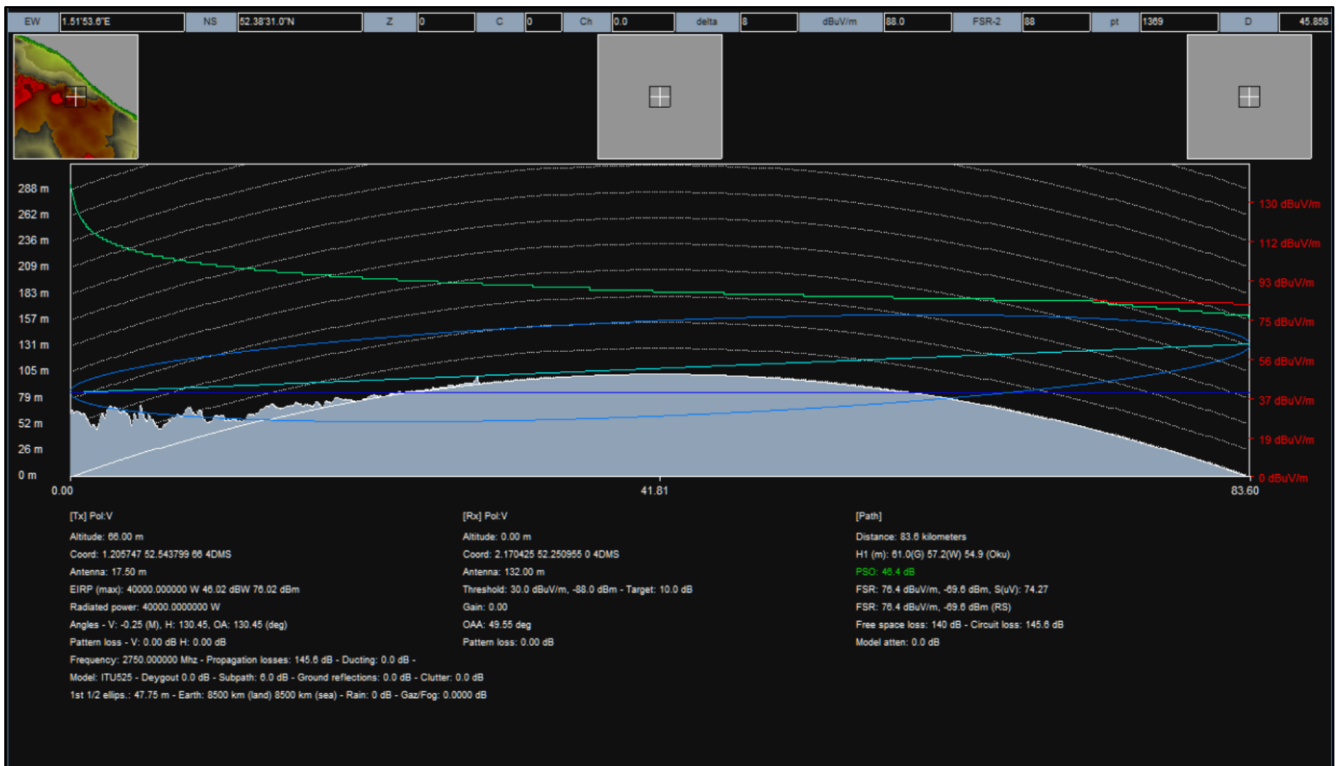
DiagramA15.1.27 Cromer Radar Propagation Model to closest point of East Anglia ONE North
