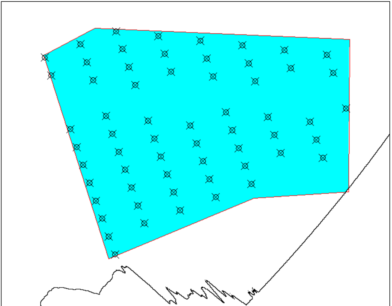
DiagramA15.1.12 Trimingham RLoS to 244m Turbines
