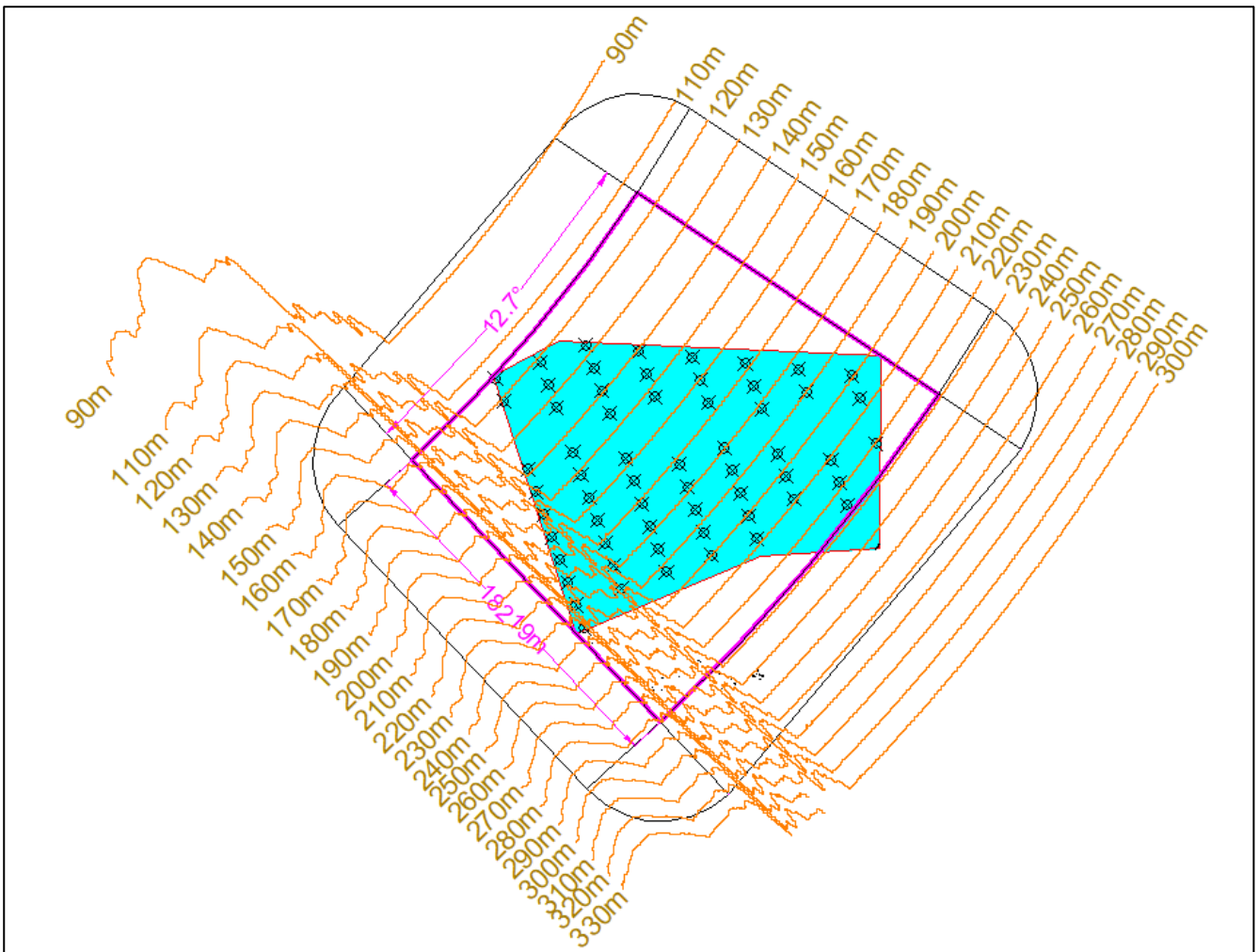
DiagramA15.1.18 Trimmingham 244m turbine buffer RLoS contours
