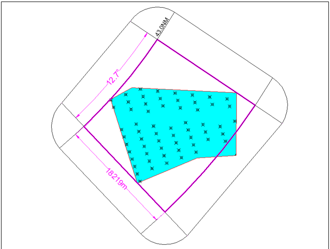
DiagramA15.1.17 Trimingham 244m turbine NAIZ buffer
