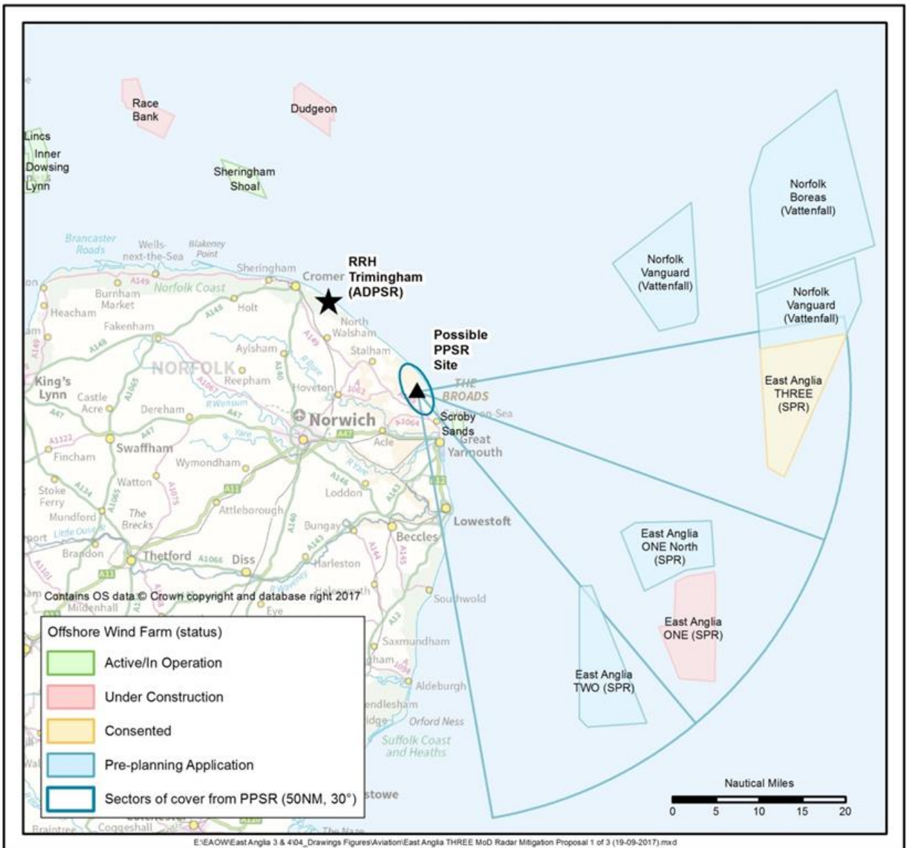
Diagram A15.1.22 Aveillant Theia sectors of cover
