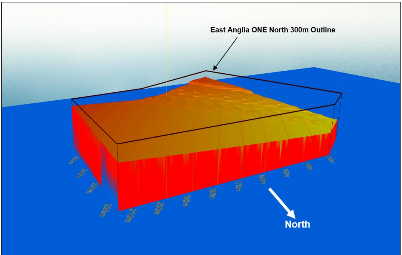
DiagramA15.1.24 3D representation of Cromer PSR RLoS to East Anglia ONE North, viewed from the north-east
