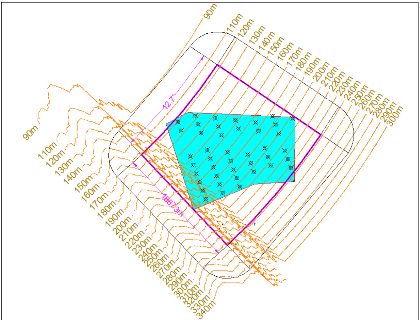
Diagram A15.1.21 Trimmingham 300m turbine buffer RLoS contours
