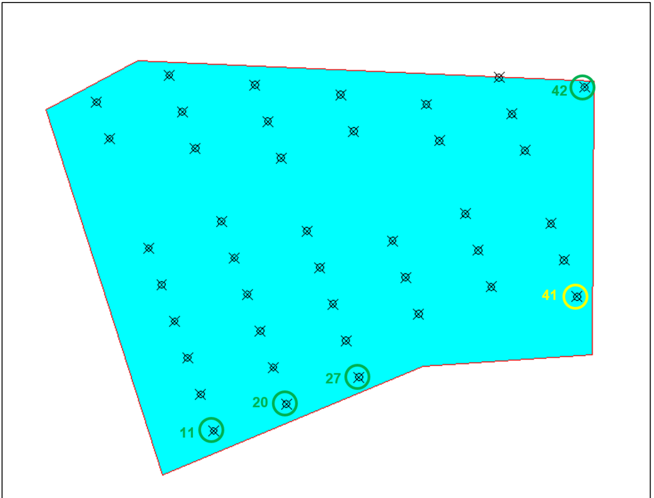
DiagramA15.1.34Cromer radar Pd of 300m turbines with reduced antenna gain
