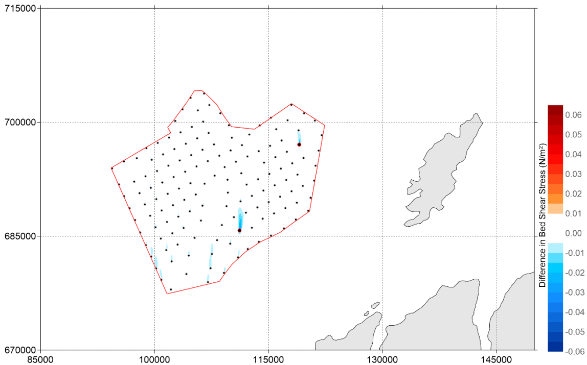
Figure 5-138: Difference in Bed shear stress ( N/m^2 ) between 'Baseline' and '15 MW - Even Spread layout' during neap tide (positive means increase of bed shear stress by layout and vice versa) - peak flood
