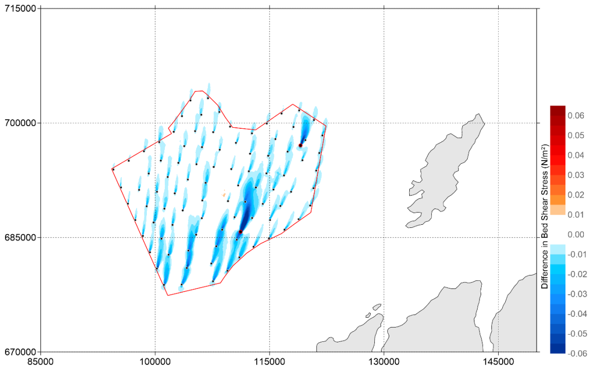
Figure 5-141: Difference in Bed shear stress ( \text{N/m}^2 ) between 'Baseline' and '24 MW - Dense Perimeter layout' during spring tide (positive means increase of bed shear stress by layout and vice versa) - peak flood
