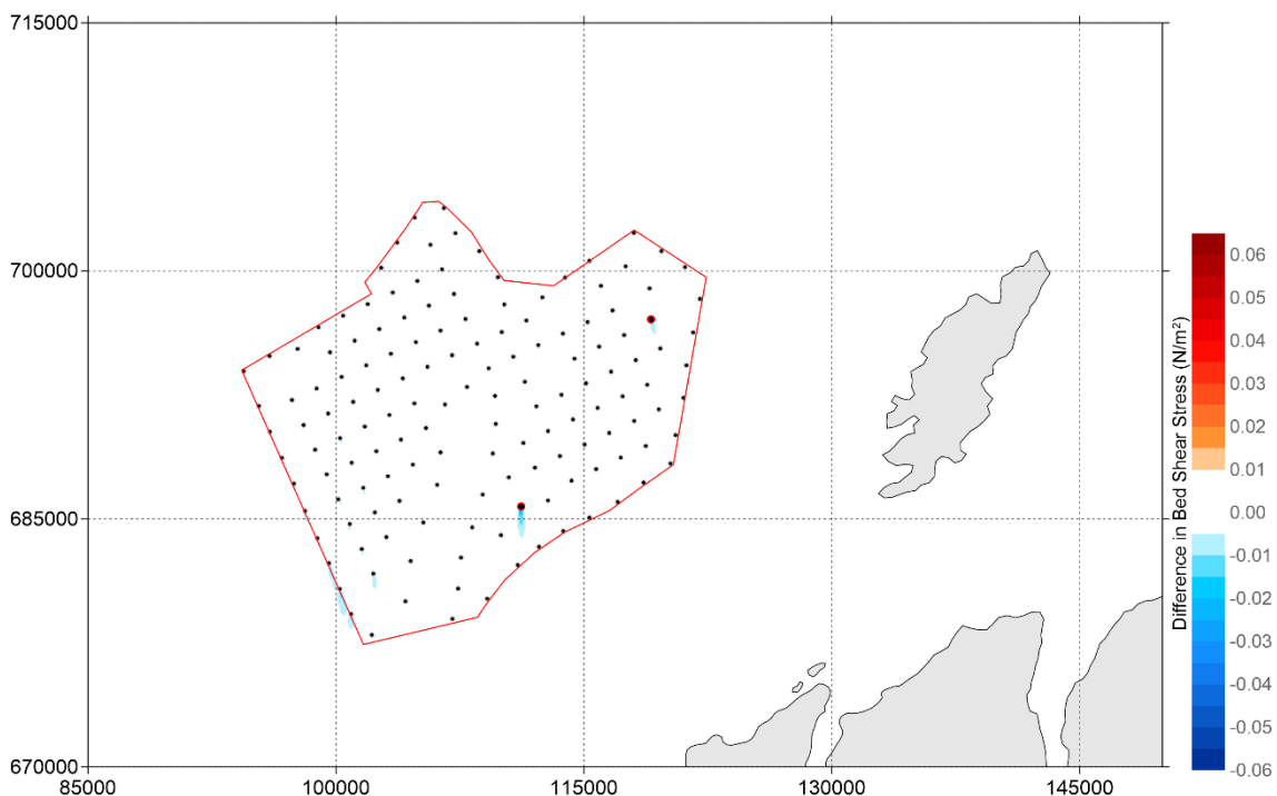
Figure 5-139: Difference in Bed shear stress ( N/m^2 ) between 'Baseline' and '15 MW - Even Spread layout' during neap tide (positive means increase of bed shear stress by layout and vice versa) - peak ebb
