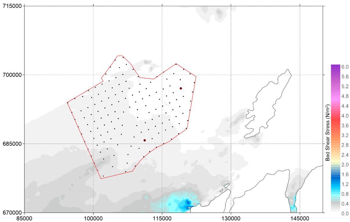
Figure 5-119: 15 MW - Even Spread layout - Bed shear stress during neap tide - peak ebb (Local model)
