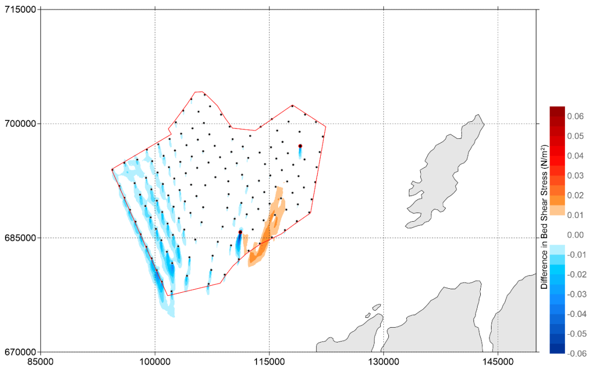
Figure 5-137: Difference in Bed shear stress ( \text{N/m}^2 ) between 'Baseline' and '15 MW - Even Spread layout' during spring tide (positive means increase of bed shear stress by layout and vice versa) - peak ebb
