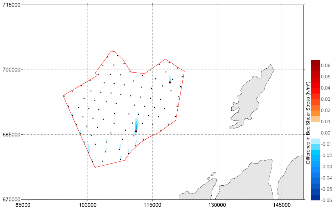
Figure 5-143: Difference in Bed shear stress ( \text{N/m}^2 ) between 'Baseline' and '24 MW - Dense Perimeter layout' during neap tide (positive means increase of bed shear stress by layout and vice versa) - peak flood
