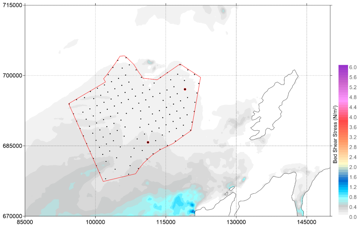
Figure 5-118: 15 MW - Even Spread layout - Bed shear stress during neap tide - peak flood (Local model)
