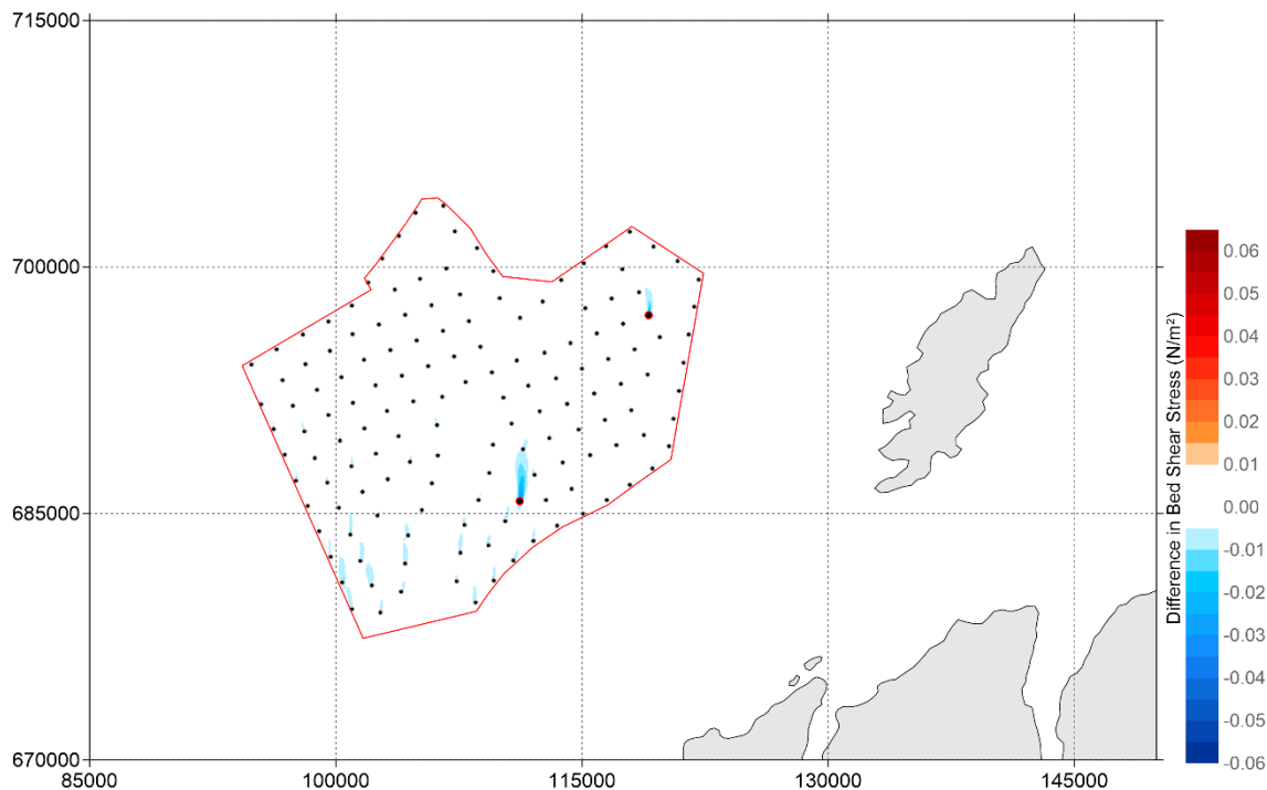
Figure 5-133: Difference in Bed shear stress ( \text{N/m}^2 ) between 'Baseline' and '15 MW - Dense Perimeter layout' during neap tide (positive means increase of bed shear stress by layout and vice versa) - peak flood
