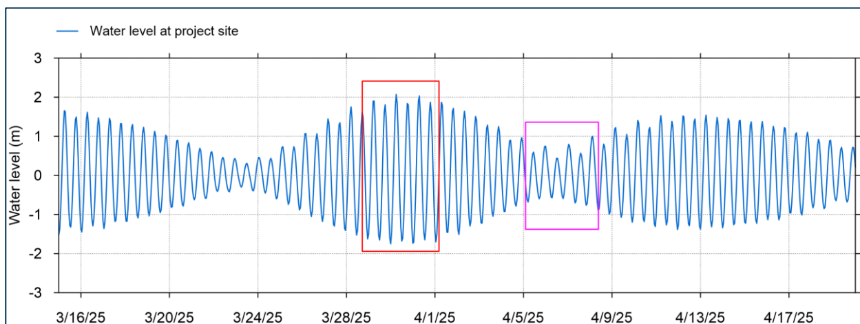
Figure 5-39: Modelled water levels at the WFD (red frame indicates spring tides and purple frame indicates neap tide)
