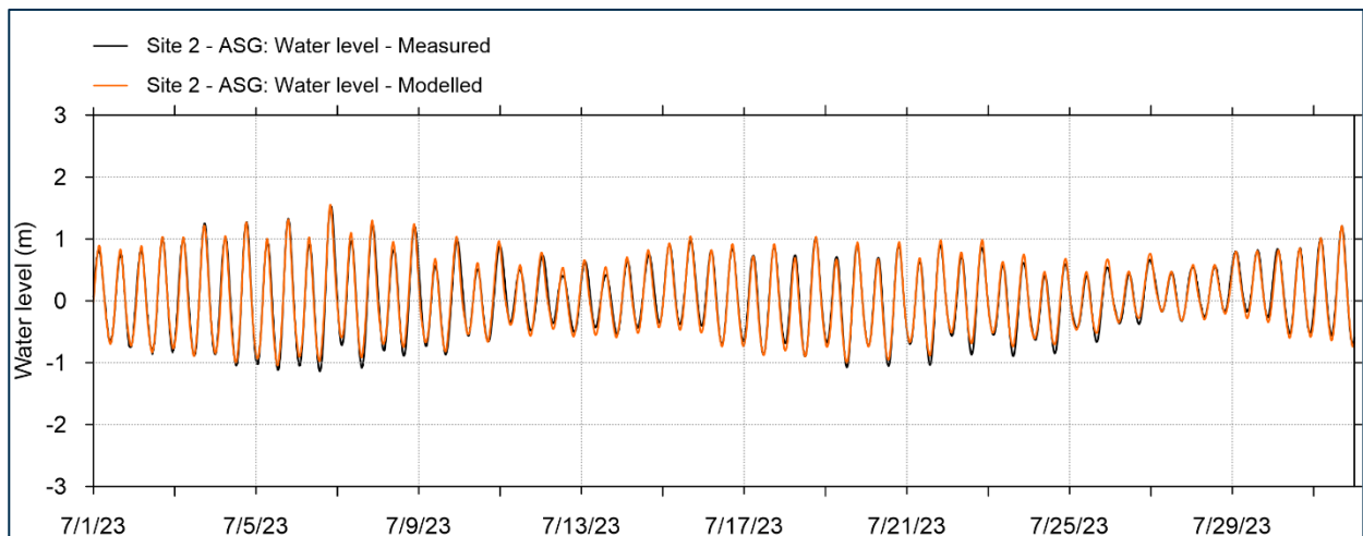
Figure 5-11: Time series comparison between simulated vs observed water levels at Site 2 - ASG in July 2023 (Regional model)
