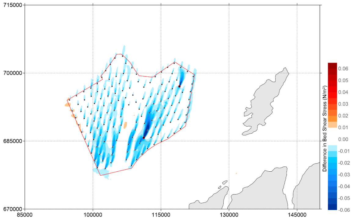
Figure 5-131: Difference in Bed shear stress ( \text{N/m}^2 ) between 'Baseline' and '15 MW - Dense Perimeter layout' during spring tide (positive means increase of bed shear stress by layout and vice versa) - peak flood
