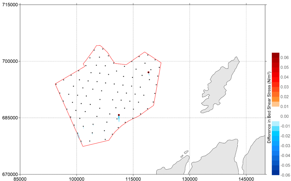
Figure 5-144: Difference in Bed shear stress ( \text{N/m}^2 ) between 'Baseline' and '24 MW - Dense Perimeter layout' during neap tide (positive means increase of bed shear stress by layout and vice versa) - peak ebb
