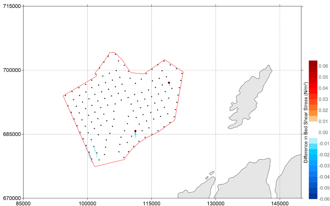
Figure 5-134: Difference in Bed shear stress ( \text{N/m}^2 ) between 'Baseline' and '15 MW - Dense Perimeter layout' during neap tide (positive means increase of bed shear stress by layout and vice versa) - peak ebb
