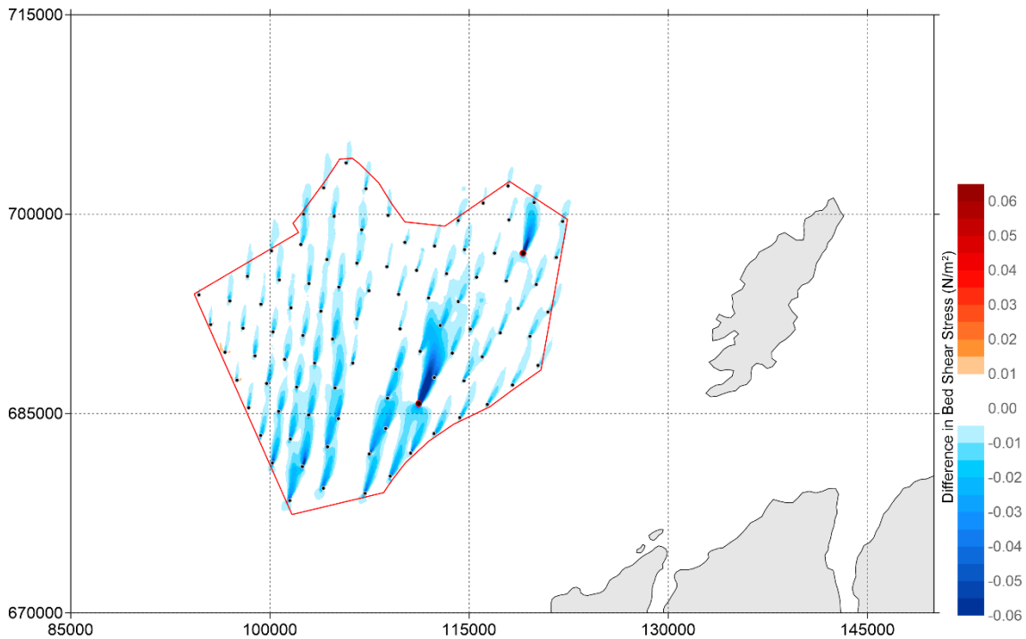
Figure 5-146: Difference in Bed shear stress ( \text{N/m}^2 ) between 'Baseline' and '24 MW - Even Spread layout' during spring tide (positive means increase of bed shear stress by layout and vice versa) - peak flood
