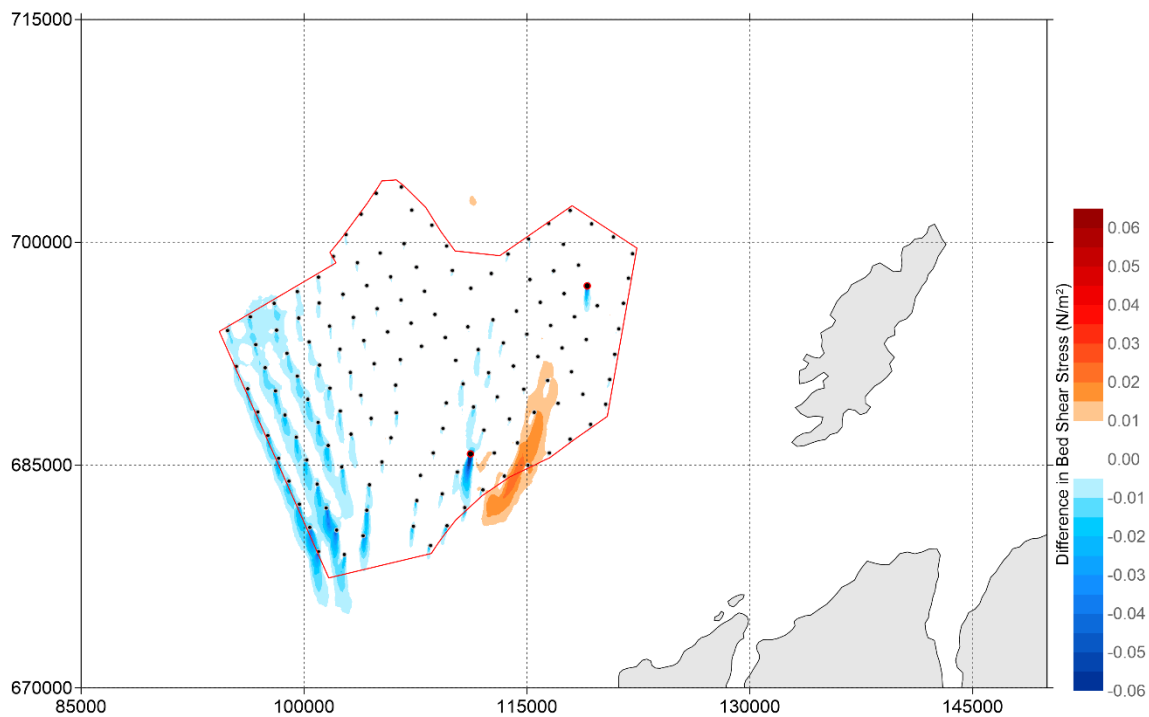
Figure 5-132: Difference in Bed shear stress ( \text{N/m}^2 ) between 'Baseline' and '15 MW - Dense Perimeter layout' during spring tide (positive means increase of bed shear stress by layout and vice versa) - peak ebb
