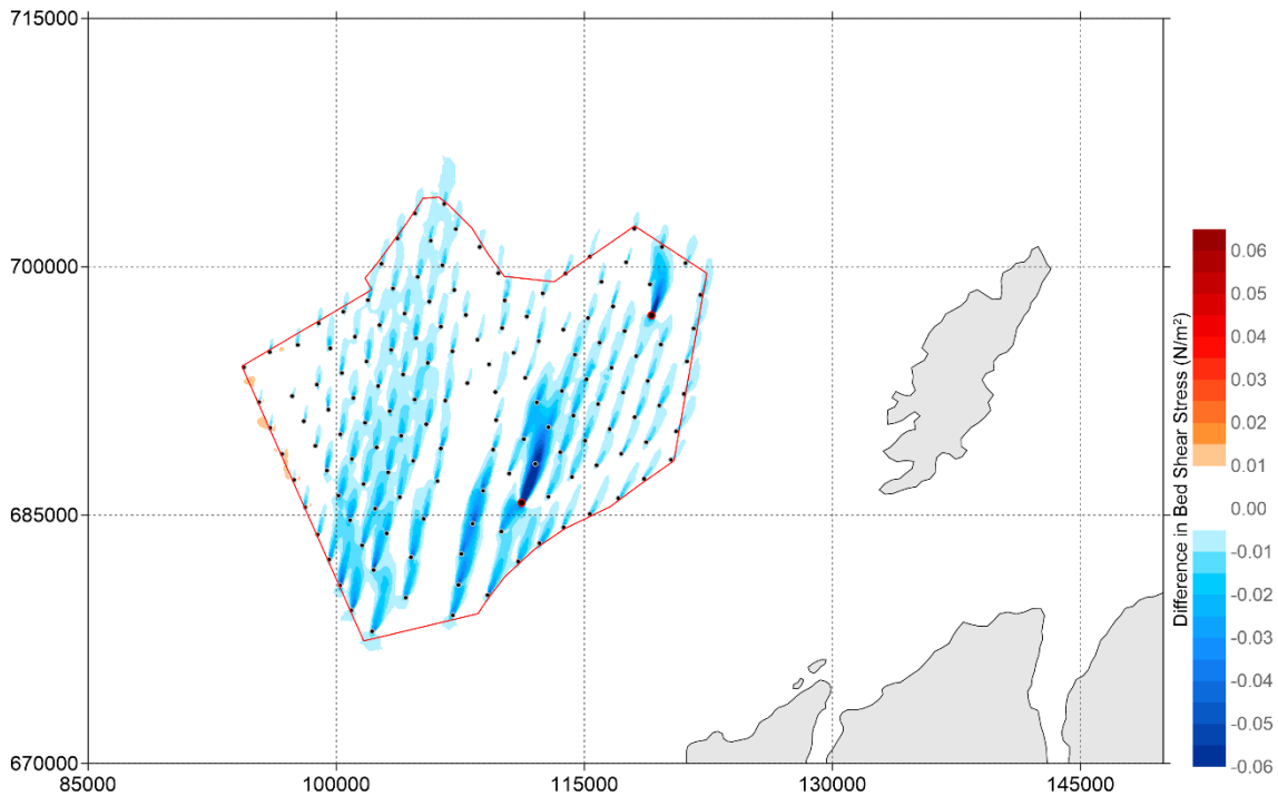
Figure 5-136: Difference in Bed shear stress ( \text{N/m}^2 ) between 'Baseline' and '15 MW - Even Spread layout' during spring tide (positive means increase of bed shear stress by layout and vice versa) - peak flood
