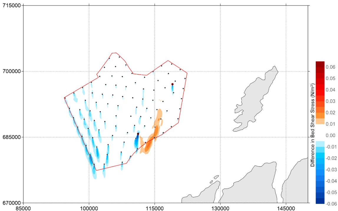
Figure 5-142: Difference in Bed shear stress ( \text{N/m}^2 ) between 'Baseline' and '24 MW - Dense Perimeter layout' during spring tide (positive means increase of bed shear stress by layout and vice versa) - peak ebb
