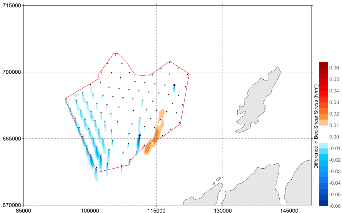
Figure 5-147: Difference in Bed shear stress ( \text{N/m}^2 ) between 'Baseline' and '24 MW - Even Spread layout' during spring tide (positive means increase of bed shear stress by layout and vice versa) - peak ebb
