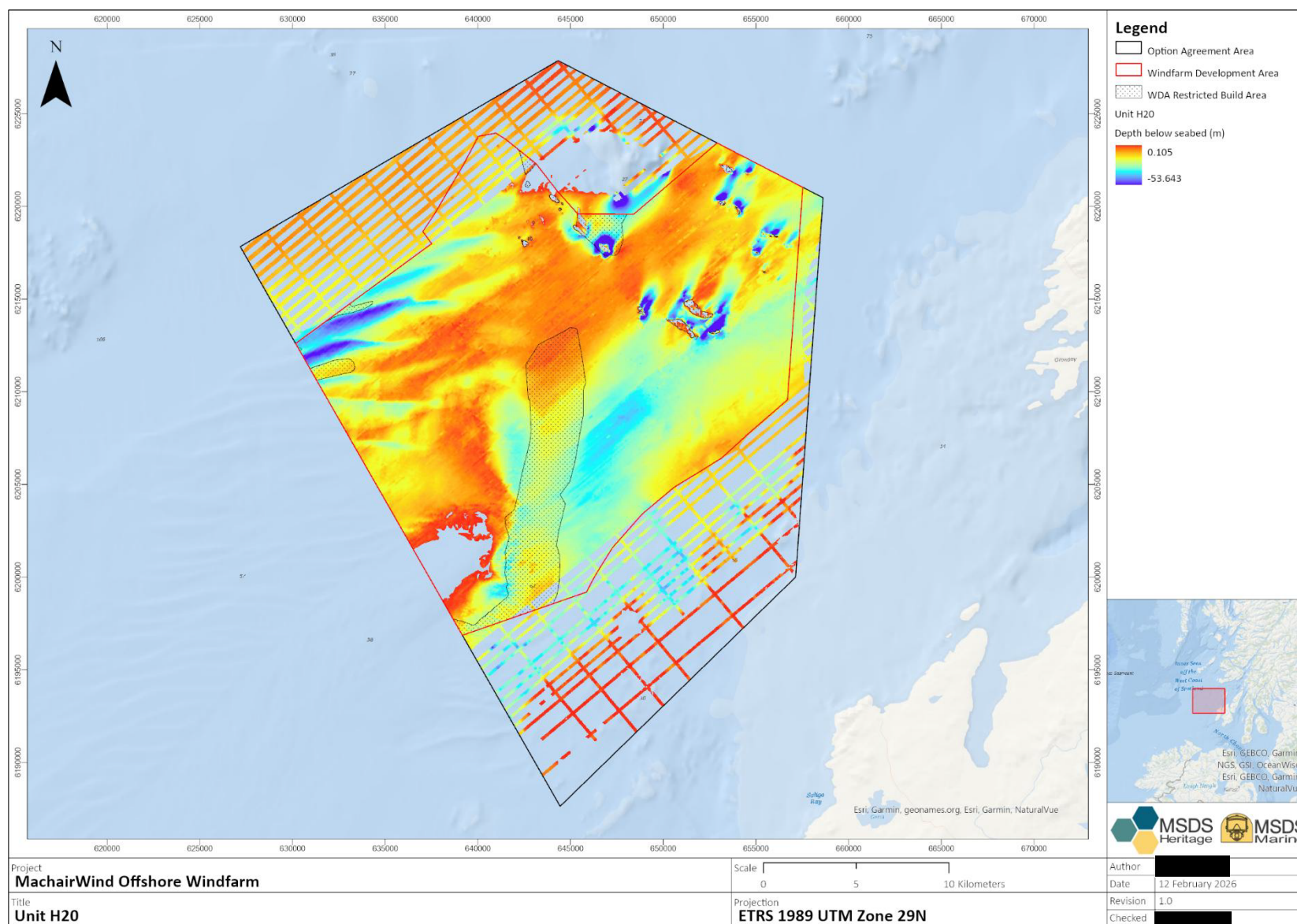
Figure 22 Sulmara H20 surface
