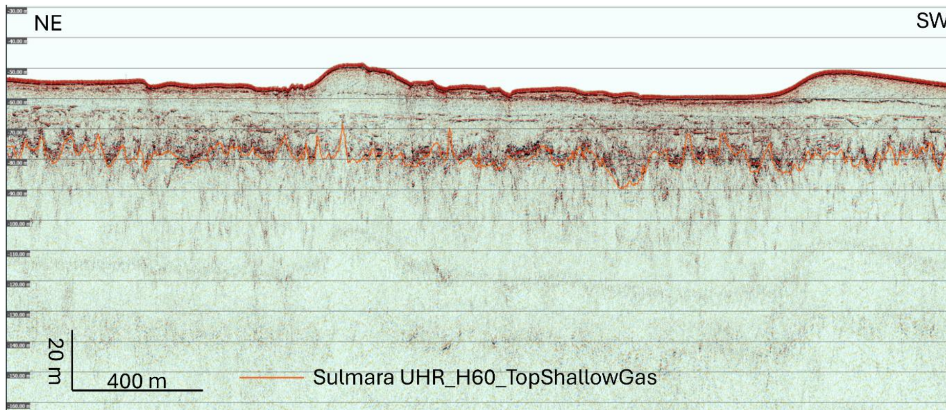
Figure 7 Fugro UHR data example of Shallow Gas limiting imaging below 20-30 m below seabed (line MCWA018B)
