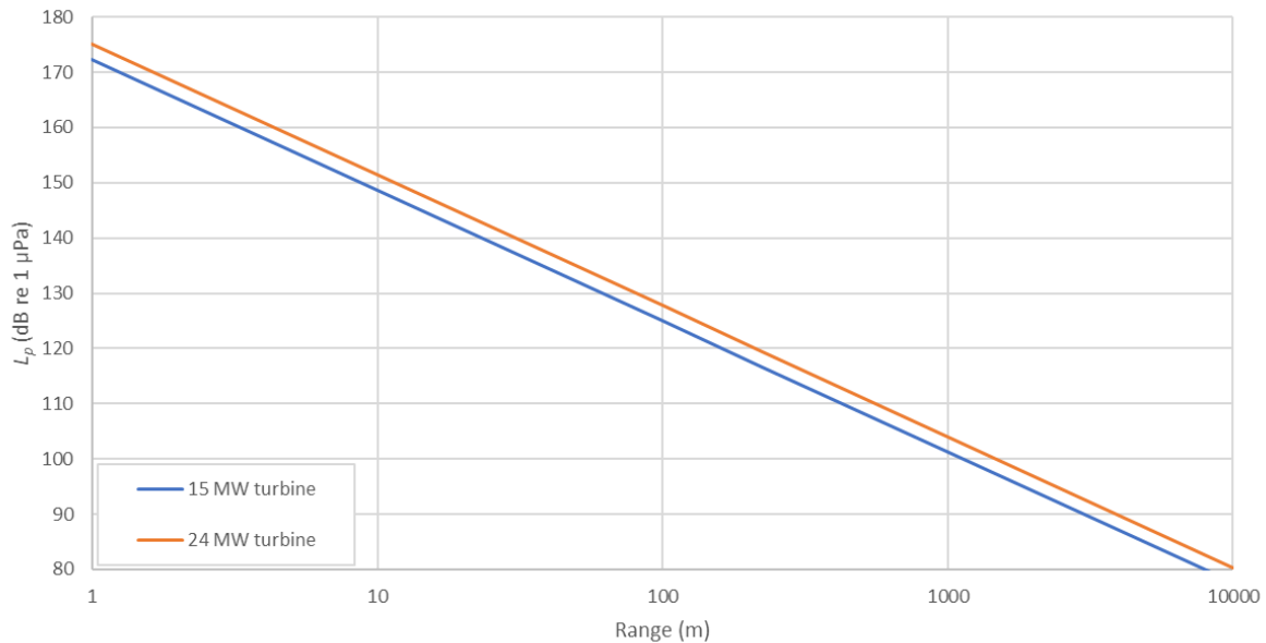
Figure 5.2: Predicted unweighted L_p from operational WTGs using the calculation from Tougaard et al. (2020).
